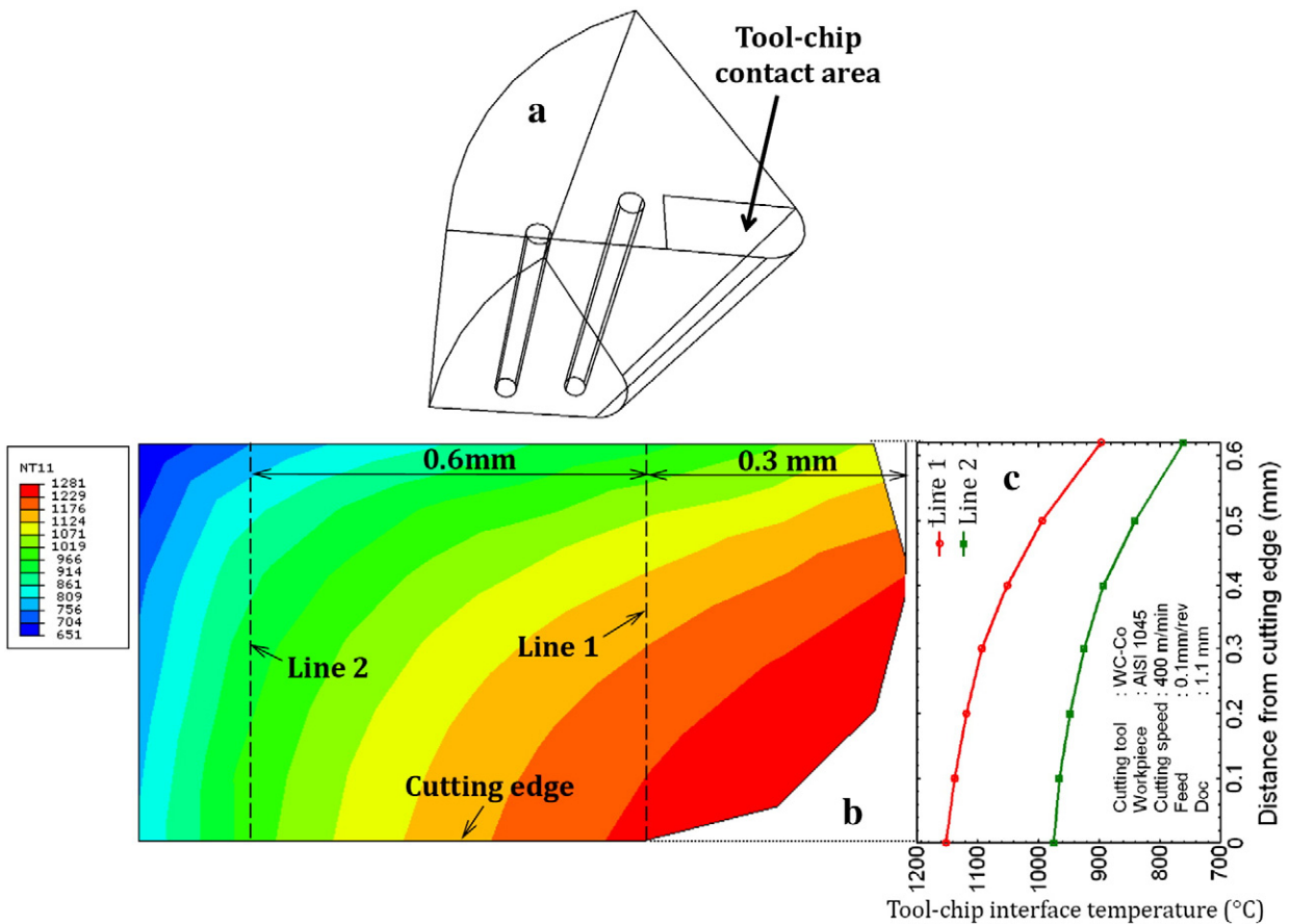
Fig. 4. Cutting tool: (a) definition of tool–chip contact area, (b) rake face temperature distribution, (c) temperature profiles on the rake face [14,24] ( V_c = 400 m/min, f = 0.1 mm/rev, a_p = 1.1 mm, after end of cut).
