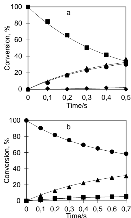
Figure 2. Hydride ligand exchange data for the interconversion of 8 and 9 in the presence of 75-fold excess of py, as probed through the selective excitation of (a) H a of 8 and (b) H c of 9 , over the defined observation period; the observation points are listed as H a (■), H b (◆), H c (●) and H d (▲) as defined in Scheme 4. The solid lines correspond to simulated changes that yield the rate constants in the text.
