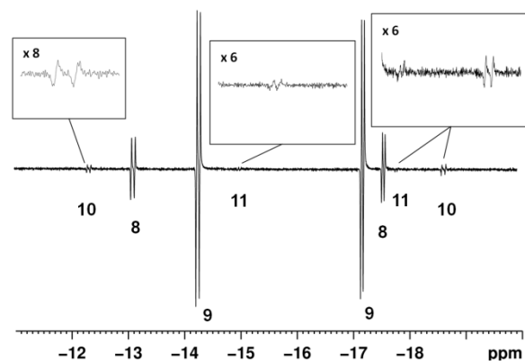
Figure 3. NMR spectra showing characteristic hydride resonances of 8 , 9 , 10 and 11 (as indicated) observed during reaction of 1 in d 4 -methanol with p -H 2 and 45-fold excess of pyridine at 273 K.
