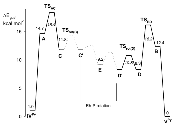
Figure 5. Energy profile (gas phase energies in kcal/mol) of the isomerization pathway of Scheme 9.
