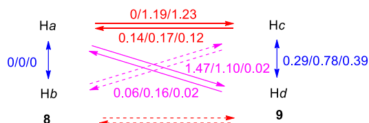
Scheme 5. The three numbers on each arrow are the exchange rates in s -1 relative to the solution with an 8-fold, 75-fold and 173-fold excess of py.
