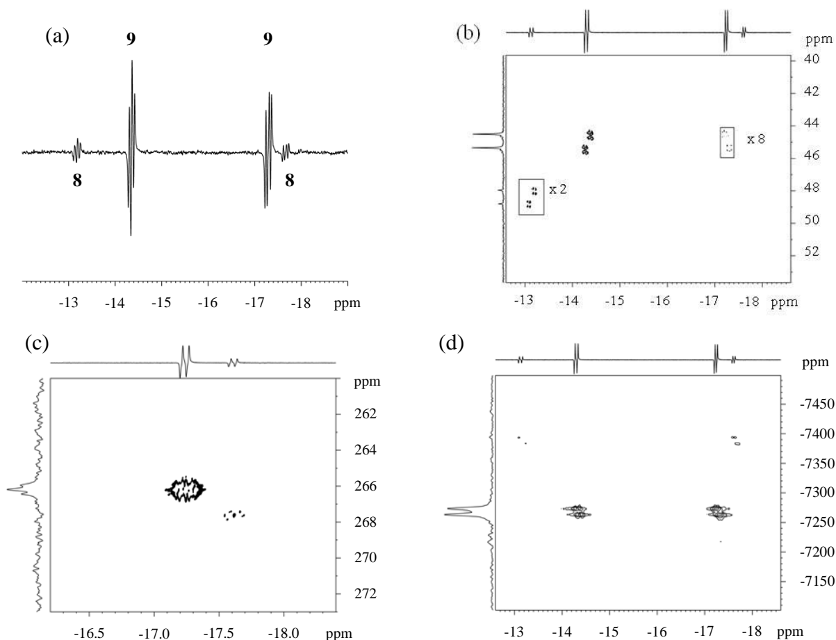
Figure 1. NMR spectra showing characteristic resonances of 8 and 9 (as indicated) observed during reaction of 2 in d_4 -methanol with p\text{-H}_2 and 75 equiv of pyridine at 263 K: (a) p\text{-H}_2 -enhanced ^1\text{H} NMR spectrum showing the hydride region; (b) ^1\text{H}\text{-}^{31}\text{P} HMQC NMR spectrum collected using ^{15}\text{N} labeled pyridine; (c) ^{15}\text{N} labeled, ^1\text{H}\text{-}^{15}\text{N} HMQC NMR spectrum; (d) ^1\text{H}\text{-}^{103}\text{Rh} HMQC NMR spectrum (in (b) the inset boxes reflect vertical expansions of x 2 and x 8 relative to the baseline).
