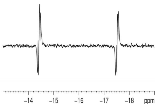
Figure 4. p - \text{H}_2 enhanced ^1\text{H} NMR spectrum showing the hydride region of 12 observed during reaction of 1 in d_4 -methanol with p - \text{H}_2 and acetonitrile at 273 K.
