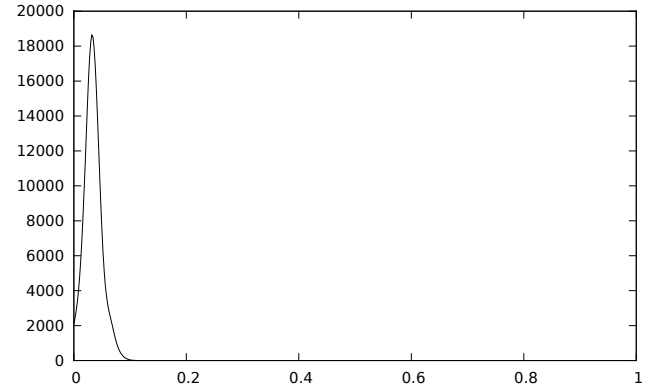
(b) Mean energy evolution
