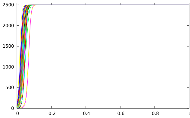
(c) Centroid evolution with 50 random initial data (the same as in (A))
