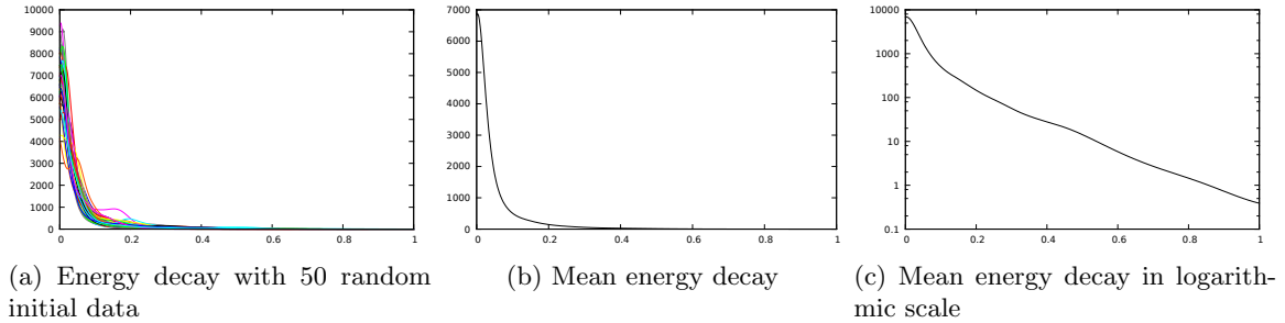
Figure 8: Energy decay for a randomly generated symmetric interaction matrix for 50 agents.
