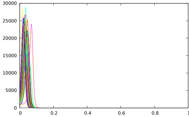
(a) Energy evolution with 50 random initial data
