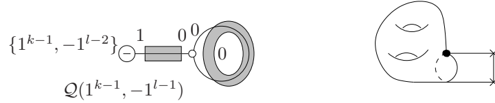
FIGURE 12. Configuration \mathcal{C}_4 for \mathcal{Q}(1^k, -1^l) in genus g \geq 1 and l \geq 2
