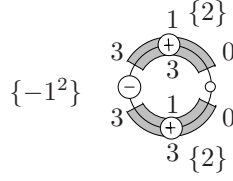
FIGURE 5. Decorated ribbon graph symmetry
