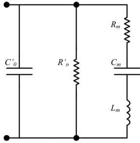
Figure 6. MBVD equivalent circuit of an effective 350 \mu\text{m} length and 50 \mu\text{m} width TFEAR. ( f_r = 14.35 \text{ MHz} , C'_0 = 1.88 \text{ pF} , R'_p = 9 \text{ k}\Omega , R_m = 375 \Omega , C_m = 12.8 \text{ fF} and L_m = 9.6 \text{ mH} )
