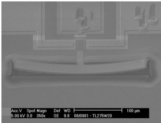
Figure 2. SEM view of a 275 \mu\text{m} length and 20 \mu\text{m} width TFEAR.
