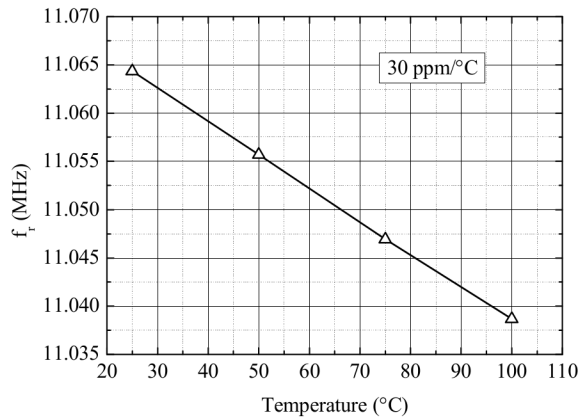
Figure 10. Frequency shift versus temperature in uncompensated temperature mode ( f_{r0} = 11.06435 MHz)
