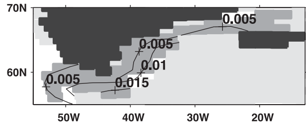
FIG. 14. Regression of low-pass-filtered ( T_c = 10 yr) salinity anomalies on the isopycnal surface 27\sigma_0 onto the SAM index, when the latter leads by 65 yr. Contour interval is 0.005 psu. The gray shaded areas indicate that the regression is 10% significant. The light shading indicates grid points where the regression is not computed, as the density of 27\sigma_0 is reached less than 60% of the year.
