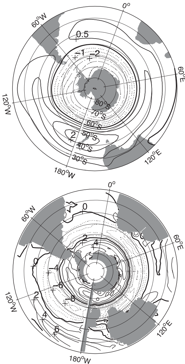
FIG. 4. (top) The SAM pattern, represented by the first EOF of the yearly SLP anomalies south of 20°S. The EOF time series (SAM index) is normalized, and the contour interval is 0.5 hPa. (bottom) Regression of annual anomalies of Ekman pumping on the SAM index. Contour interval is 2 m yr -1 . Dashed lines correspond to negative values and the thick lines to zero.
