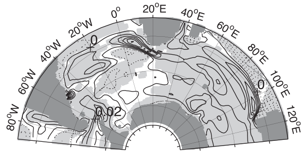
FIG. 5. Regression of annual anomalies of the averaged salinity between 0 and 100 m onto the SAM index when the SAM leads by 1 yr. Contour interval is 0.01 psu; dashed lines correspond to negative values. The shaded areas indicate that the regression is 5% significant.
