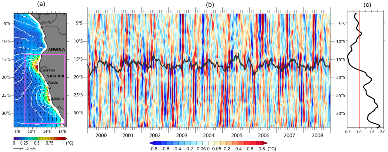
Figure 1. (a) Benguela upwelling region: subseasonal (see section 2 for the filtering procedure) SST variability (color shading, ^{\circ}\text{C} ), mean wind vector (arrows, m/s), and wind variability (contour, m/s) over the period 2000–2008. The pink rectangle indicates the region of interest of the present study. (b) Hovmuller diagram of the SST subseasonal anomalies ( ^{\circ}\text{C} ) along the African coast, from the equator to 34^{\circ}\text{S} , averaged over the coastal fringe of 150 km based on the OI TMI land mask. (c) Ratio of the scale-averaged wavelet power over the 2\text{--}30\text{ day}^{-1} frequency band to those over the 30\text{--}90\text{ day}^{-1} frequency band estimated for the SST anomalies shown in Figure 1b. It illustrates that south of ABFZ the SST experiences relatively higher-frequency variability than north of ABFZ. Black line in Figure 1b shows the position of the ABFZ defined as the latitude where the SST meridional gradient is the maximum. Note that Veitch et al. [2006] suggest that over the 100–250 km coastal band the ABFZ is more diffuse relative to near-coastal regions (30 km offshore). The SST and wind data are derived from the TMI and QuikSCAT satellite observations, respectively.
