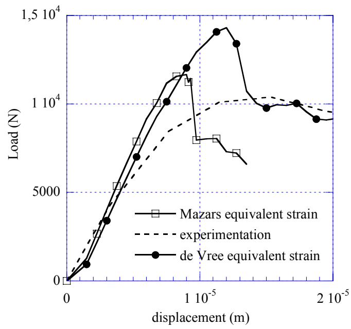
Fig 8. Nooru-Mohamed test. Comparisons of two types of damage threshold during the loading.
