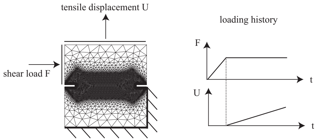
Fig 6. Nouru-Mohamed test. Mesh, boundary conditions and loading history
