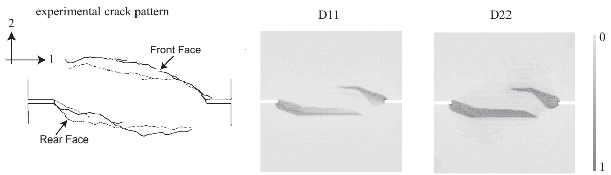
Fig 7. Nooru-Mohamed test. Experimental crack pattern. Damage fields in the direction 1 (horizontal) and 2 (vertical).
