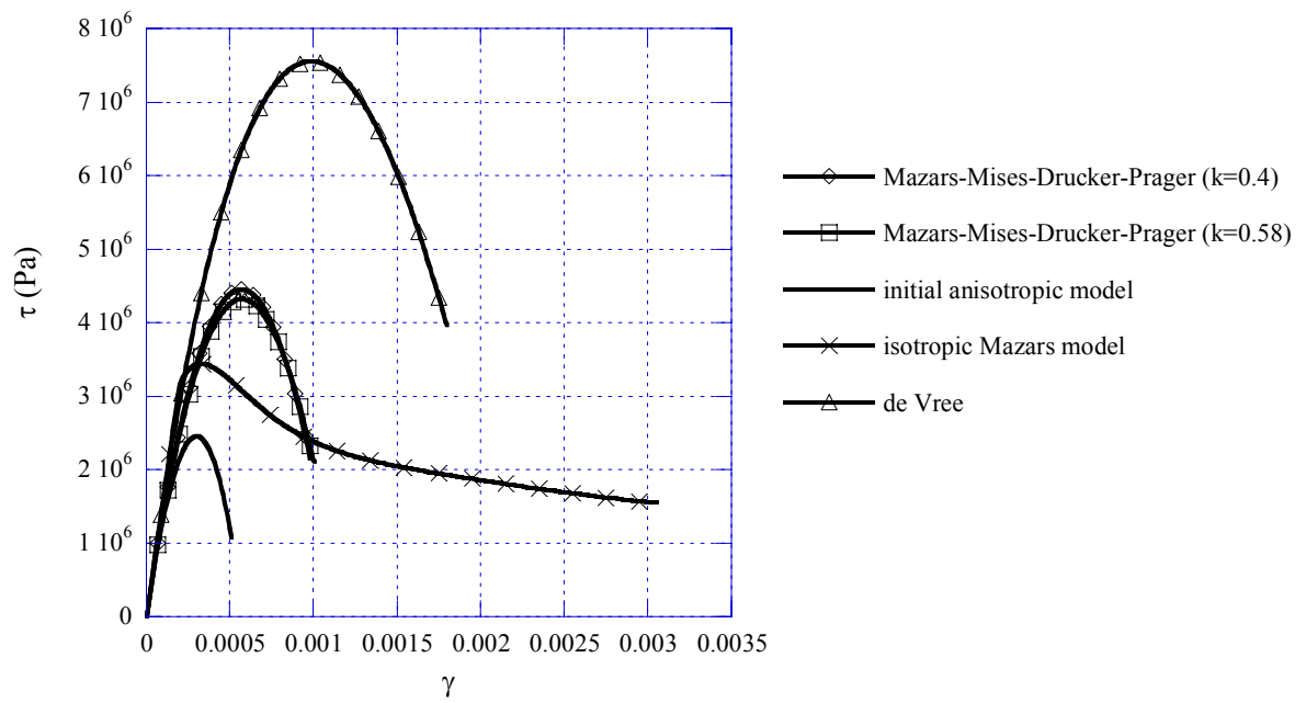
Fig 5. Shear response for the isotropic and the anisotropic damage models using the different expressions for the equivalent strains.
