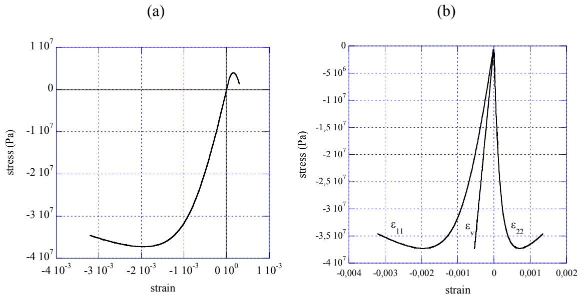
Fig 1 : Uniaxial response of the anisotropic damage model. (a) Tension/compression non symmetric feature and (b) volumic behaviour in compression ( \epsilon_v = Tr\epsilon ).
