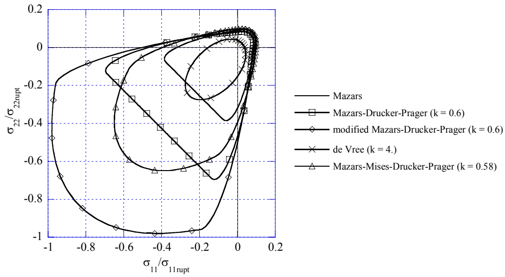
Fig 3. Elasticity domains comparisons for the different equivalent strains. The k parameter has been adjusted to obtain for each model the same responses in tension and in compression as in figure 1.
