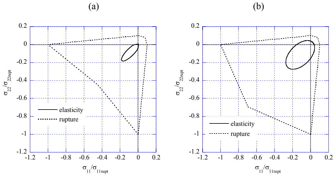
Fig 4. Elasticity domain and ultimate state at rupture for (a) the anisotropic damage model using Mazars-Mises-Drucker-Prager equivalent strain and (b) the de Vree Criterion.
