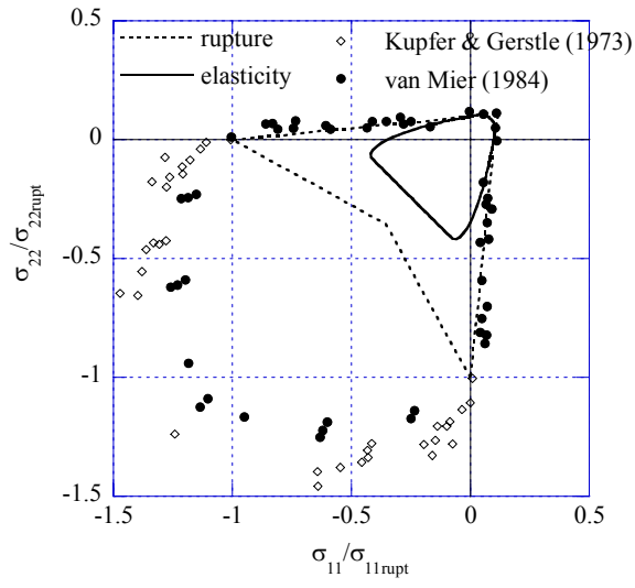
Fig 2. Elasticity domain and ultimate state at rupture for (a) the isotropic model (Mazars 1984) and (b) the initial anisotropic model using the Mazars equivalent strain.
