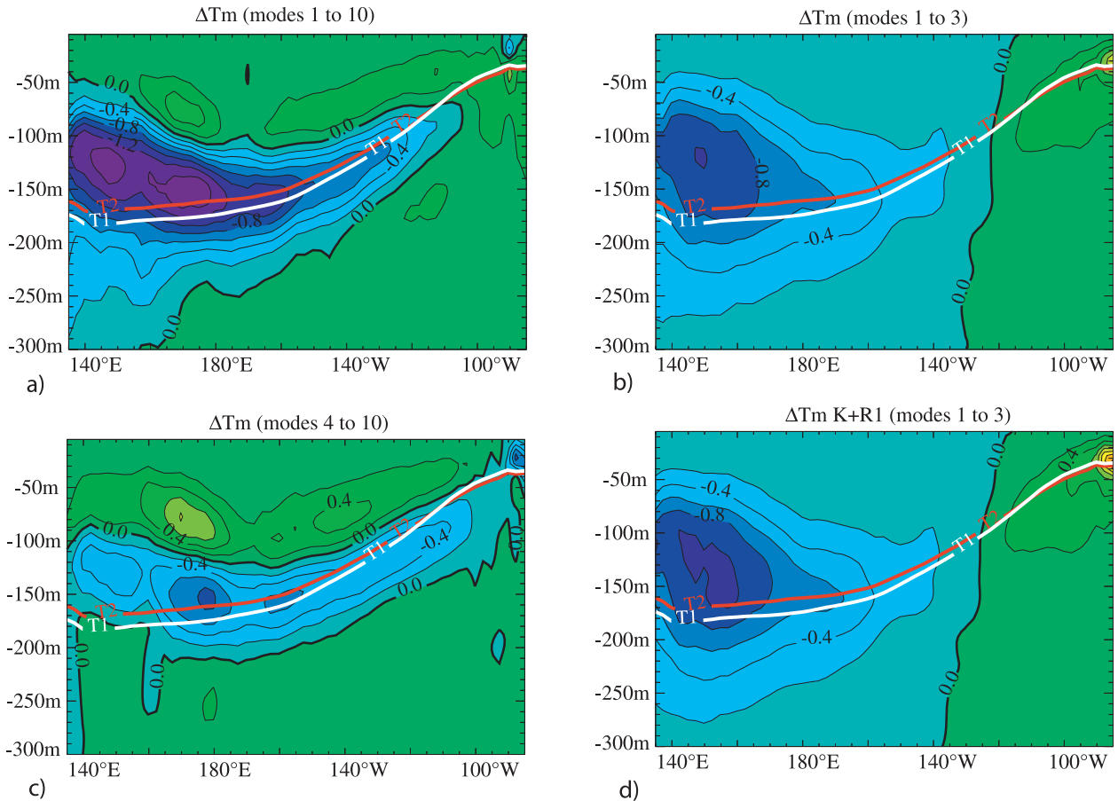
FIG. 2. Same as in Fig. 1, but for the summed-up contribution of the baroclinic modes (a) 1–10 (b) modes 1–3, (c) modes 4–10, and (d) for the contribution of the Kelvin and first meridional Rossby waves of the first three baroclinic modes.
