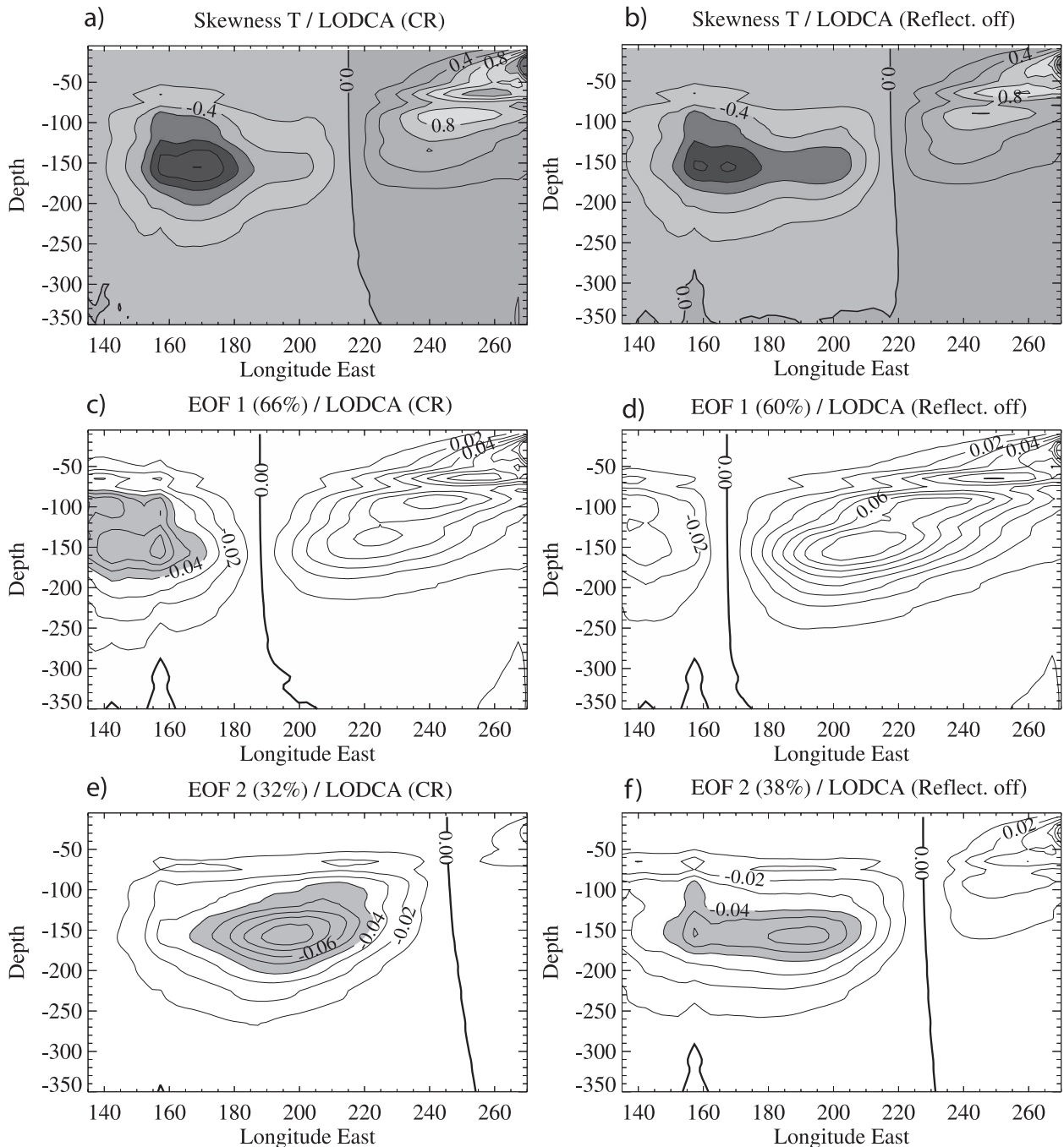
FIG. 7. Results of the linear model experiments: (a),(b) Skewness of baroclinic temperature and (c)–(f) EOF1 and EOF2 (spatial pattern) of its low-frequency component (A 7-yr low-pass filter is applied on \sum_{m=1}^3 T_m ) along the equator and as a function of depth; (left) LODCA-CR and (right) LODCA-Roff (see text). Units are in ^{\circ}\text{C} for skewness. The PC time series associated with the EOF1 and EOF2 for LODCA-CR are displayed in Fig. 4a (dashed lines).
