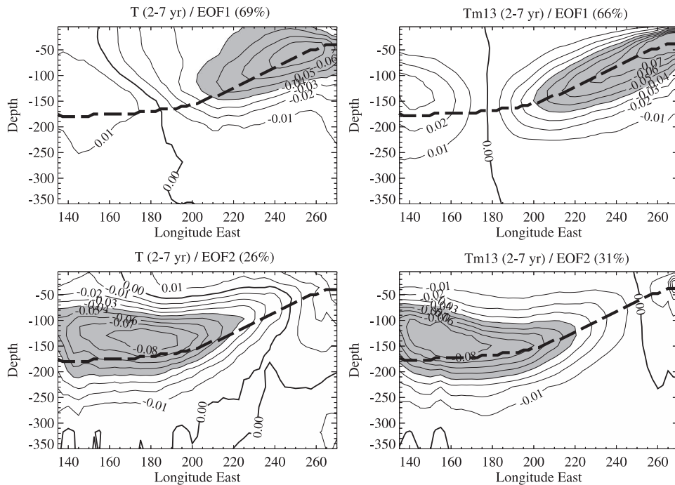
FIG. 5. Same as in Fig. 3, but for the interannual variability [i.e., data were previously bandpass filtered for frequencies between 2 and 7 ( \text{yr}^{-1} )]. The thick dashed line represents the mean thermocline depth.
