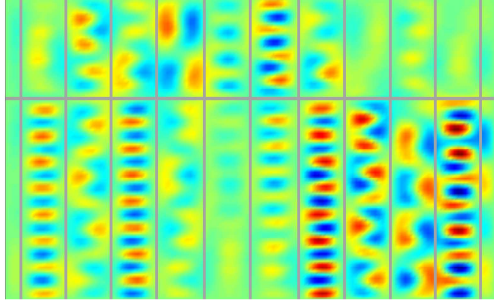
Figure 6: 288 th mode for the case 2 (ribbed plate with bridge) of frequency of 4190 Hz presenting complex vibratory phenomenon.
