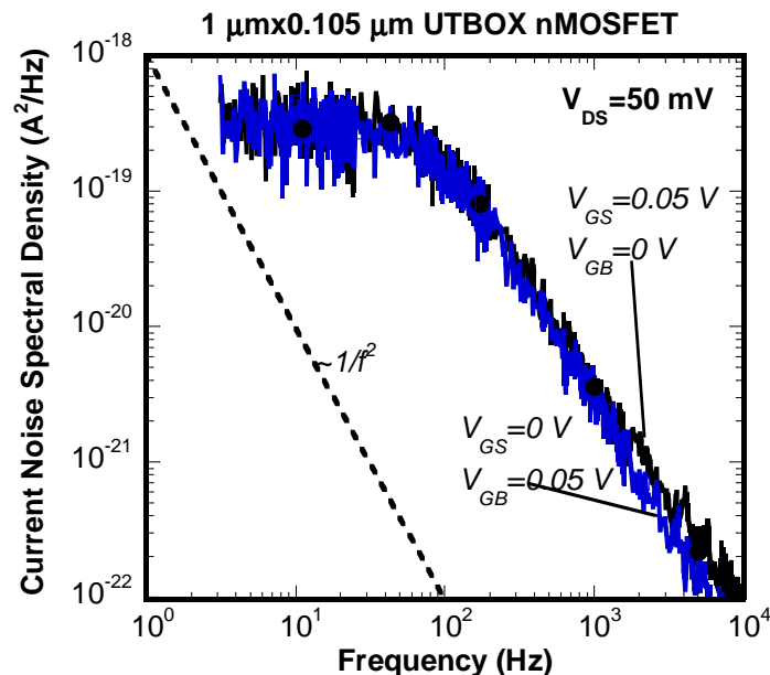
Fig. 9. Low-frequency noise spectra for a UTBOX SOI nMOSFET, operated at the front-gate with the back-gate V_{GB} at 0 V or at the back-gate with the front-gate at 0 V.
