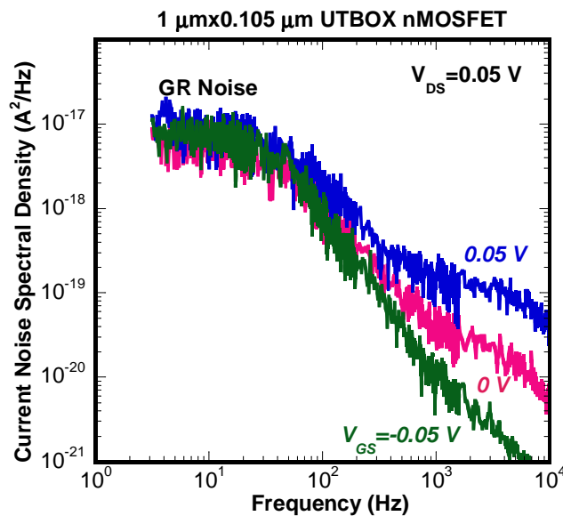
Fig. 5. Low-frequency noise spectra around V_T for a 1 \mu\text{m} \times 0.105 \mu\text{m} UTBOX SOI nMOSFET, exhibiting generation-recombination noise around 10 Hz.
