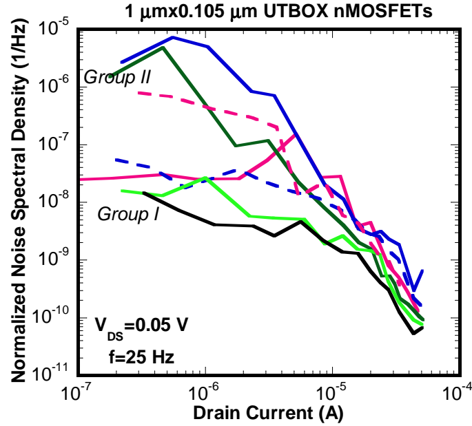
Fig. 6. Normalized noise current spectral density versus drain current at f=25 Hz and in linear operation for a set of FD SOI nMOSFETs, aligned across the vertical diameter in the center of an UTBOX wafer.
