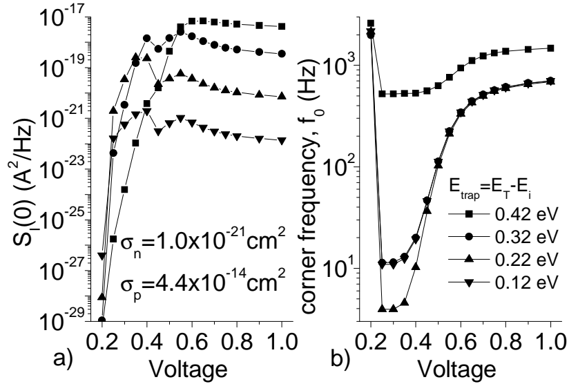
Fig. 8. Simulated plateau amplitude (a) and corner frequency (b) as a function of the front-gate voltage at zero back-gate, corresponding with different trap level positions with respect to the intrinsic Fermi level E_i . An electron capture cross section of 1.0 \times 10^{-21} cm 2 and a hole cross section \sigma_p = 4.4 \times 10^{-14} cm 2 has been considered in the calculations. The existence of minority traps, such as the one analyzed in this figure can boost the noise variability. In this case, the peak seen at low voltages in (b) reflects the fact of a small number of electrons in the silicon and that the term related to hole capture and emission cannot be neglected
