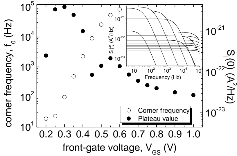
Fig. 7. Simulated corner-frequencies f_0 and plateau value S_I(0) of the Lorentzian component as a function of the front-gate voltage. The back-gate voltage is 0 V. Inset: detail of the variation of the corresponding Lorentzian spectra with gate voltage. E_T - E_i = 0.16 eV; \sigma_n = 2.5 \times 10^{-19} cm 2 and N_T = 10^{17} cm -3 .
