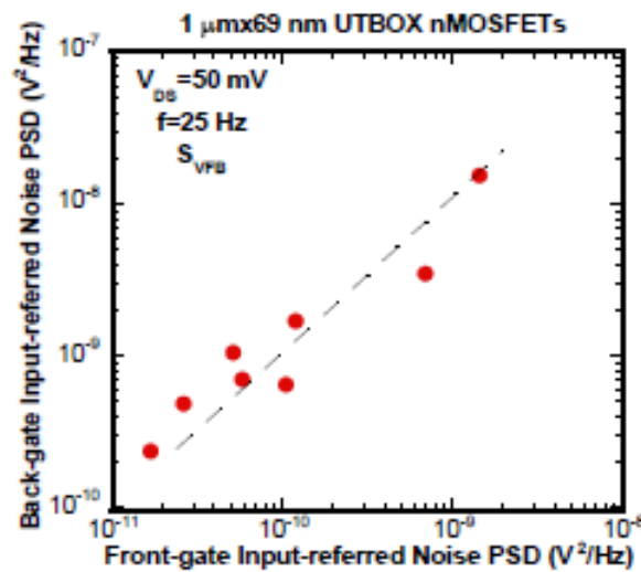
Fig. 4. Back- versus front-channel average input-referred noise PSD at flatband ( V_{GS} \sim V_T ), f = 25 Hz and V_{DS} = 50 mV for a set of 1 \mu\text{m} \times 69 nm UTBOX nMOSFETs with t_{Si} \approx 14 nm and t_{SiO_2} = 5 nm.
