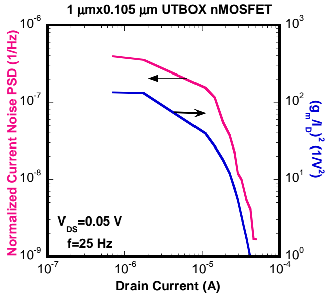
Fig. 3. Normalized current noise PSD at 25 Hz versus drain current and (g_m/I_D)^2 versus I_D in linear operation ( V_{DS}=0.05 V) for a 1 \mu\text{m} \times 0.105 \mu\text{m} UTBOX SOI nMOSFET.
