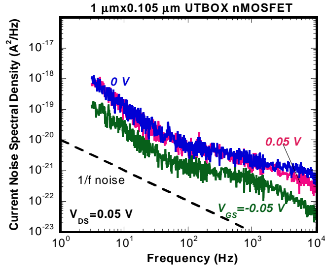
Fig. 2. Low-frequency noise spectra around V_T for a 1 \mu\text{m} \times 0.105 \mu\text{m} UTBOX SOI nMOSFET, exhibiting flicker noise around 10 Hz. The back-gate is at 0 V in depletion. The drain voltage V_{DS}=0.05 V in linear operation.
