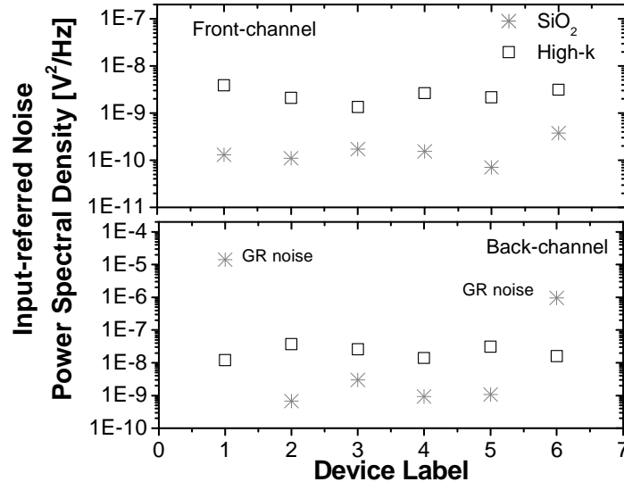
Figure 4: Front and back-channel S_{VG} for high-k and SiO 2 splits at 25 Hz.
