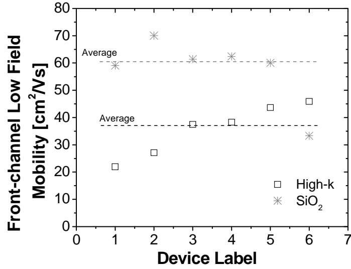
Figure 2: Front-channel low field mobility for each transistor measured along the vertical diameter of the wafer for high-k and \text{SiO}_2 splits.
