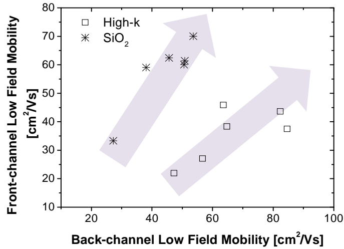
Figure 3: Correlation of front and back-channel low field mobility for high-k and \text{SiO}_2 splits.
