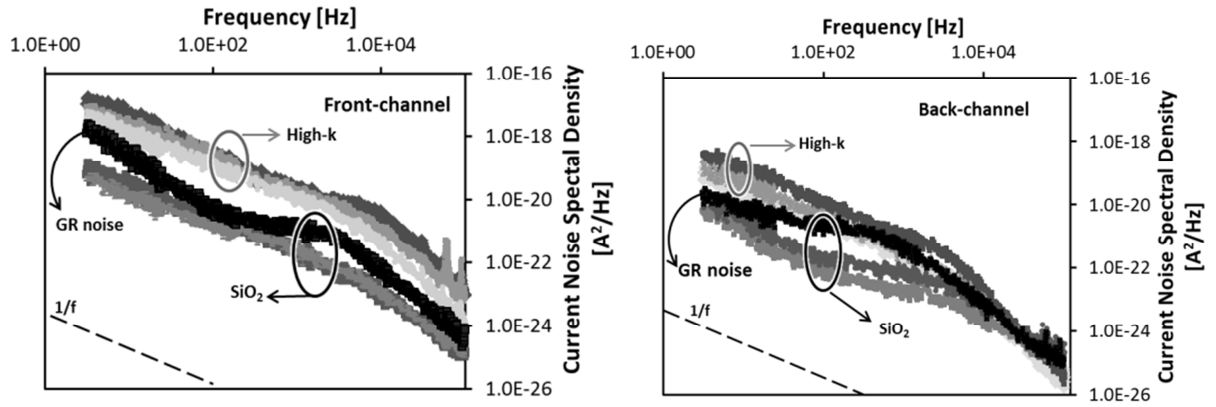
Figure 5: Front (a) and back-channel (b) current noise spectral density versus frequency for high-k and SiO 2 splits, showing the occurrence of a Lorentzian PSD in one of the spectra.
