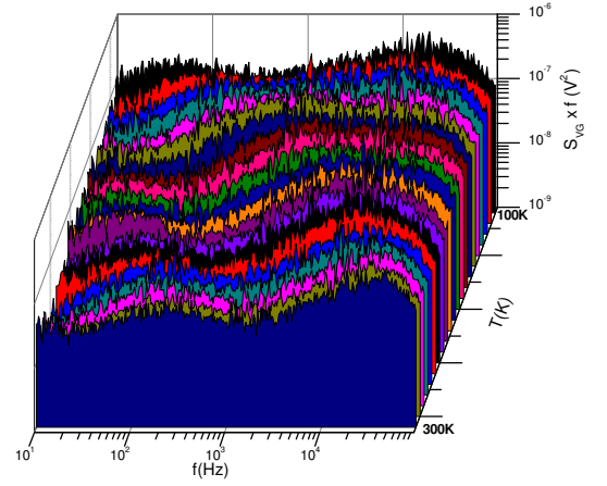
Figure 3. Frequency normalized noise spectral density versus temperature for a p-channel sSOI+CESL FinFET with L_G=60 nm.
