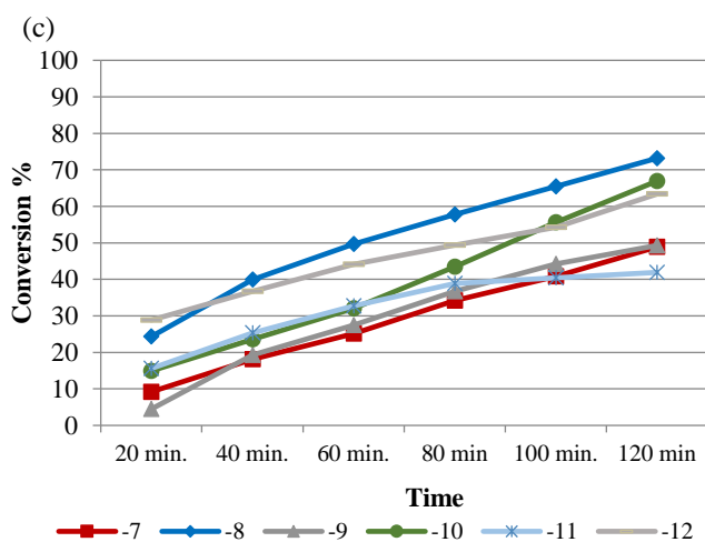
Figure 5. Catalytic activity as shown by the % conversion vs. time for the transfer hydrogenation of (a) acetophenone, (b) 4-chloro-acetophenone, (c) 4-methyl-acetophenone catalyzed by compounds 7-12 in isopropanol. Conditions: ketone/Ru/KOH, 1:0.002:10; T= 82 °C
