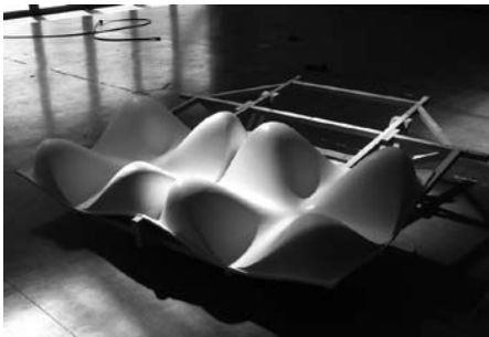
Figure 6 (a) Egg-box shape ( 2\text{ m} \times 2\text{ m} ). (b) Origami shape ( 1.8\text{ m} \times 1.8\text{ m} ).
