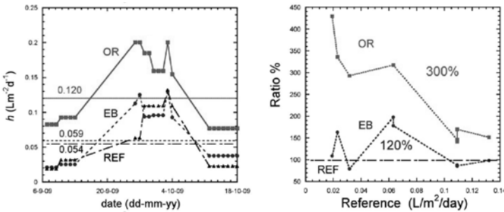
Figure 8 (a) Evolution of dew yields ( \text{Lm}^{-2}\text{day}^{-1} ) for the origami (OR, squares, full line), egg box (EB, short dashed line) and reference plane (REF, triangles, long dashed line) with mean values - horizontal lines). (b) Ratio R of the condenser to the reference plane with respect to dew yields (OR, squares, full line), (EB, dashed line). The thick lines are 100% weighting of the data.
