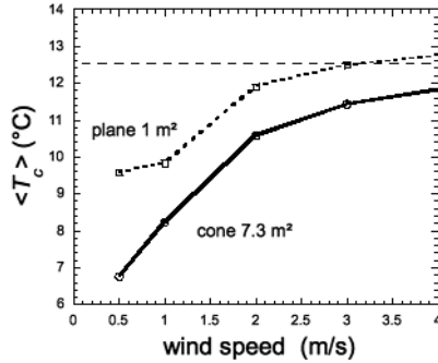
Figure 2 Averaged condenser surface temperatures \langle T_c \rangle as obtained by numerical simulation with respect to wind speed at 10 m elevation. No condensation occurs above the broken line \langle T_c \rangle > T_d = 285.5 \text{ K} ( 12.5^\circ \text{C} ), corresponding to T_a = 288 \text{ K} ( 15^\circ \text{C} ) and \text{RH} = 85\% .
