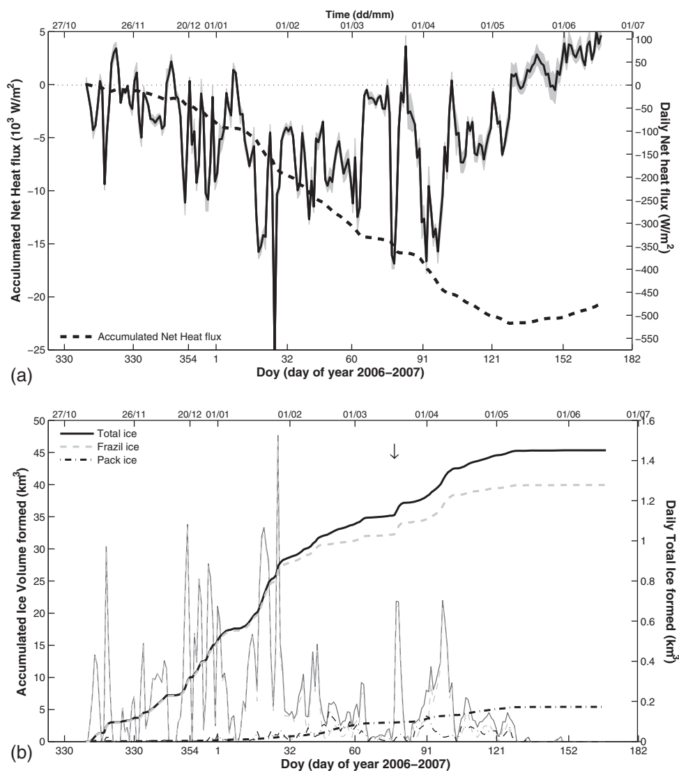
Figure 2. (top) Daily and accumulated net surface heat flux over open water ( \text{W m}^{-2} ) during 2006–2007. The gray surface identifies the \pm 1 standard deviation of the surface mean over the entire Storfjorden. (bottom) Daily (thin lines, right axis) and accumulated volume of ice formed (thick lines) for total (solid line), frazil ice (dashed line), and pack (dashed-dotted line) ice. Units are \text{km}^3 . The vertical arrow identifies the polynya opening shown in Figure 8.
