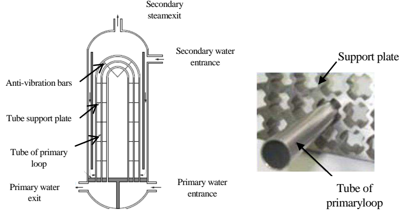
Figure 1. Steam generator
