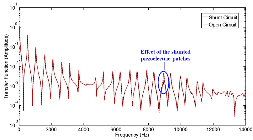
Figure 16: The forced response of the structure under white noise excitation (transfer function) tuned at 9 kHz. (Solid line)Piezoelectric patches with shunted circuit. (Dashed line)Shunt circuit open.
