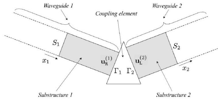
Figure 2: An illustration of the coupling between two different periodic waveguides [6].
