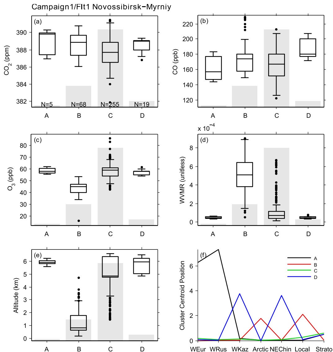
Fig. 6. (a) Box plots of median and inter-quartile range (IQR) for CO 2 concentrations measured during Flight 1 (11 April 2006) associated to each cluster (clusters A–D in abscissa, same denomination as in Fig. 5). Outliers within the IQR are included in the whiskers; outliers beyond the IQR are shown as dots. (b) Same for CO. (c) Same for O 3 . (d) Same for water vapour mixing ratio. (e) Same for altitude. (f) Cluster centroid position vector for each cluster. Gray bars indicate the population of each cluster (number of samples).
