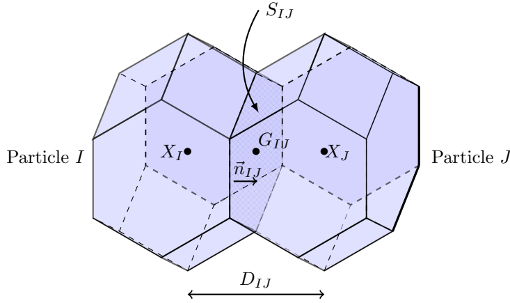
Figure 19: Contact surface between particles
