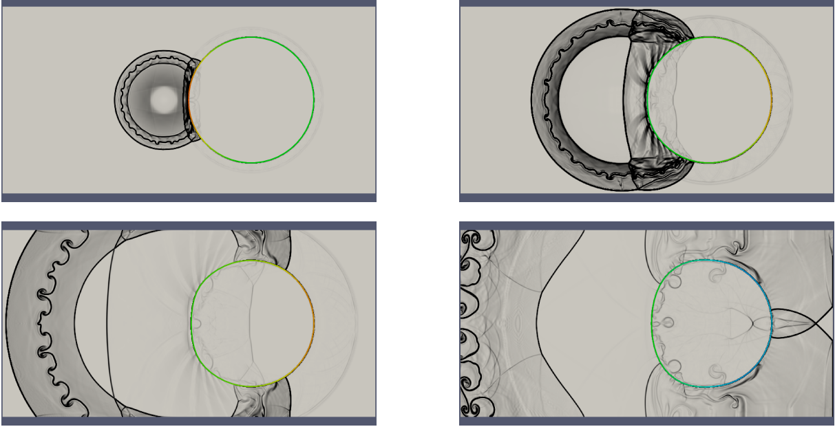
Figure 12: Density gradient in the fluid and normal stress distribution in the cylinder at four times: 2 \times 10^{-3} s, 4.7 \times 10^{-3} s, 1 \times 10^{-2} s, and 2.44 \times 10^{-2} s from left to right and top to bottom.
