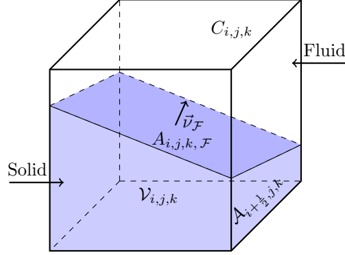
Figure 1: Illustration of a cut-cell C_{i,j,k} .
