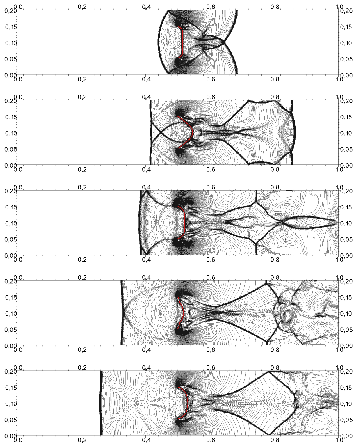
Figure 18: Density field in the fluid and solid deformation at five times: 0.07s, 0.14s, 0.21s, 0.28s, and 0.35s from top to bottom.
