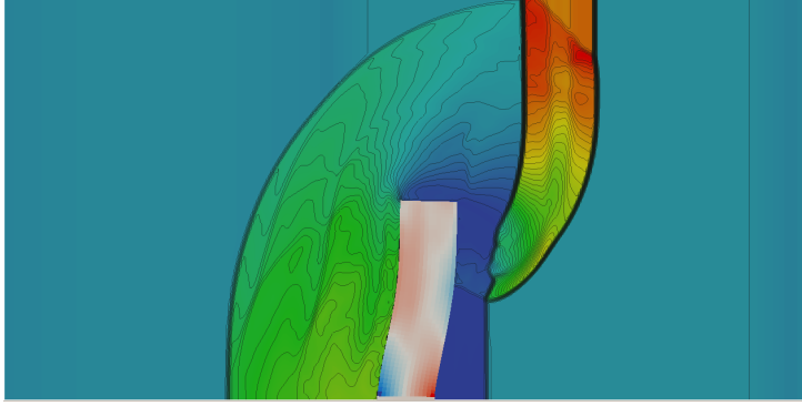
Figure 6: Normal stress in the beam and the time evolution of the pressure profile in the fluid at time t = 0.08\text{s} (50 contours in the fluid from 0 to 160Pa).
