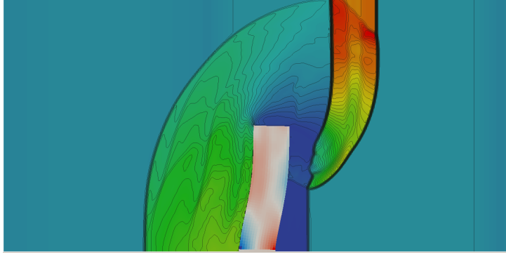
Figure 6: Normal stress in the beam and the time evolution of the pressure profile in the fluid at time t = 0.08s (50 contours in the fluid from 0 to 160Pa).
