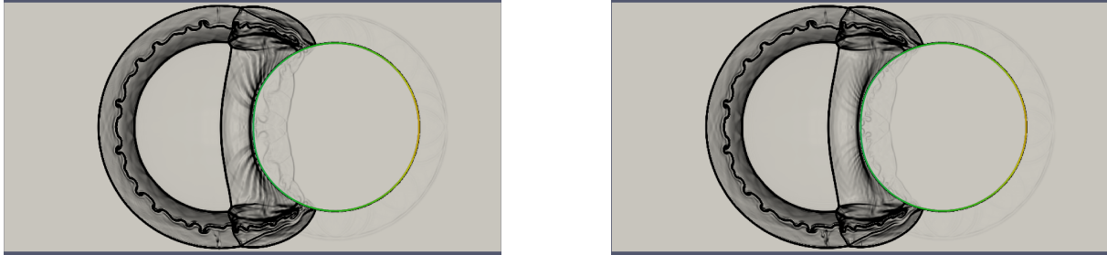
Figure 16: Density gradient in the fluid and normal stress distribution in the cylinder at time 4.7 \times 10^{-3} s for 100 solid particles (left) and 200 solid particles (right).
