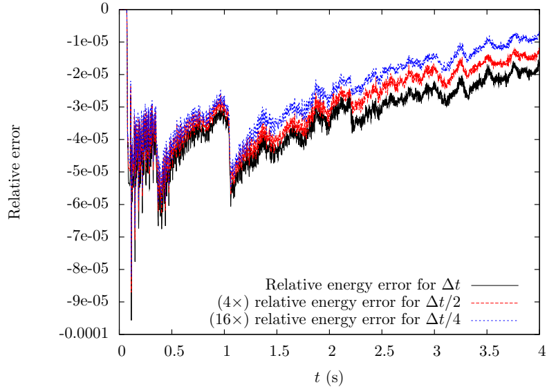
Figure 7: Relative energy conservation error as a function of time for time-steps \Delta t , \Delta t/2 (rescaled by a factor 4) and \Delta t/4 (rescaled by a factor 16).
