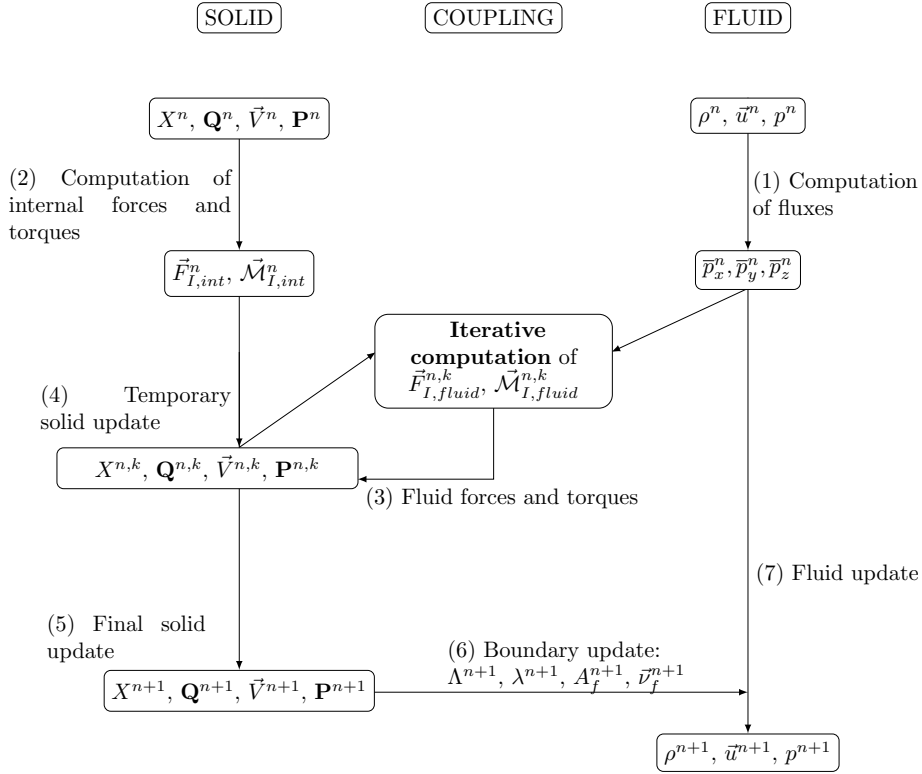
Figure 4: Structure of the time semi-implicit scheme
