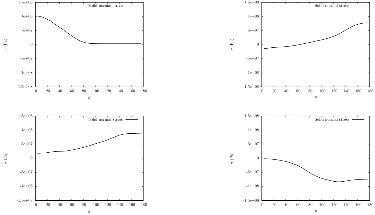
Figure 15: Normal stress profile in the cylinder as a function of azimuthal angle at four times: 2 \times 10^{-3} s, 4.7 \times 10^{-3} s, 1 \times 10^{-2} s, and 2.44 \times 10^{-2} s from left to right and top to bottom.
