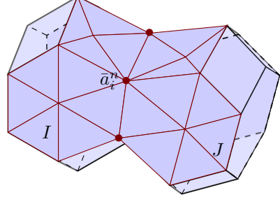
Figure 3: Reconstruction of the deformed solid boundary.
