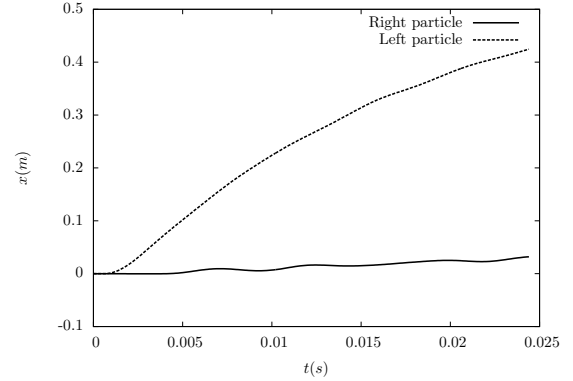
Figure 14: x -coordinate of the center of mass of the solid particle closest to the explosion (left particle) and of the solid particle farthest to the explosion (right particle) as a function of time.
