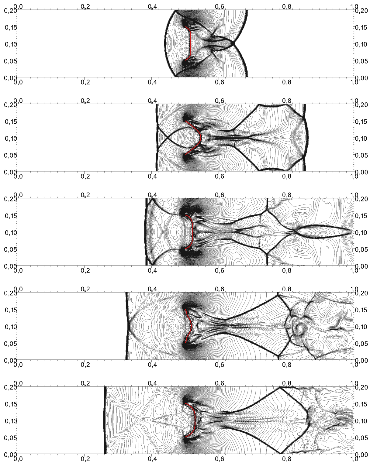
Figure 18: Density field in the fluid and solid deformation at five times: 0.07s, 0.14s, 0.21s, 0.28s, and 0.35s from top to bottom.
