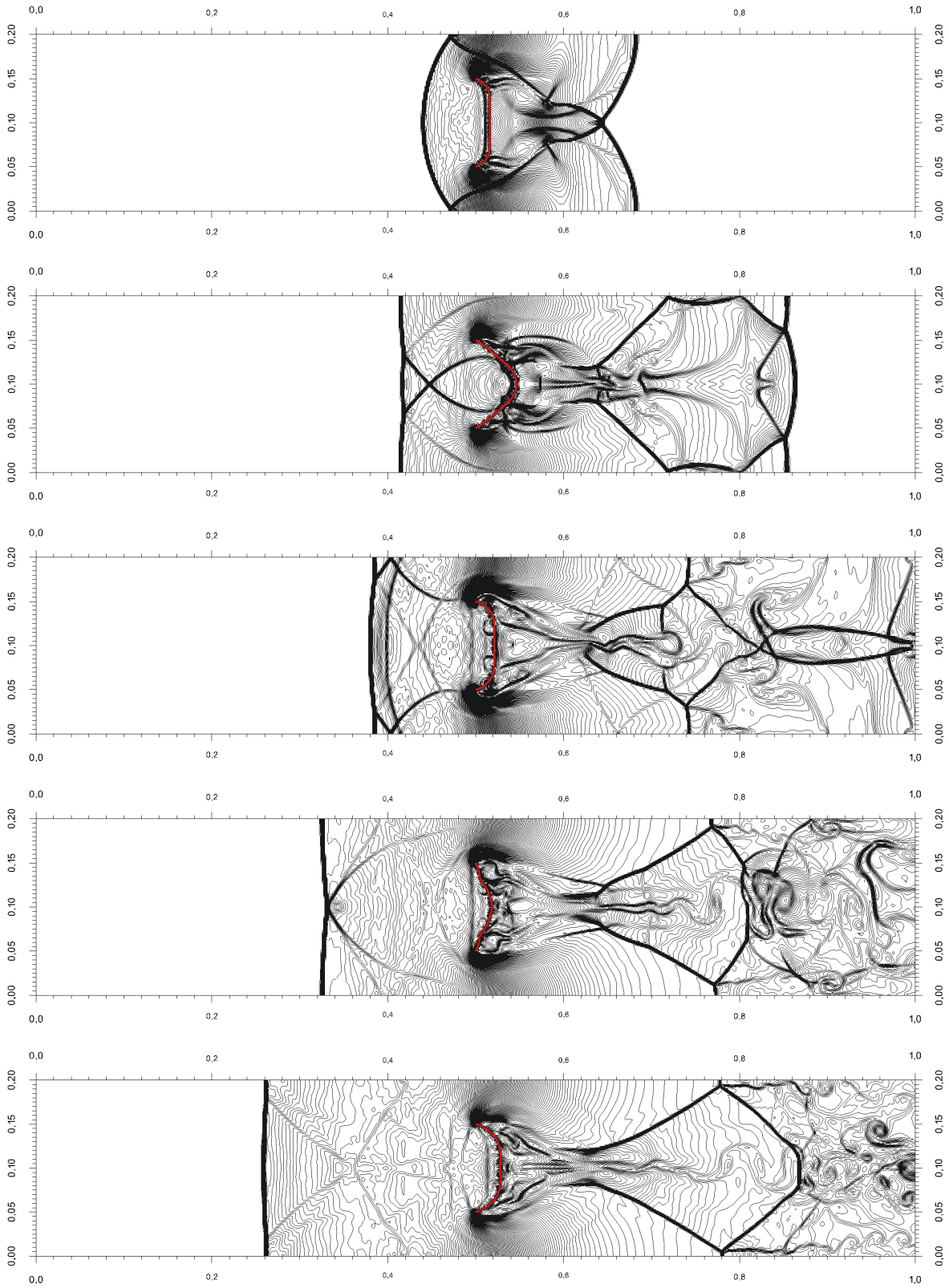
Figure 18: Density field in the fluid and solid deformation at five times: 0.07s, 0.14s, 0.21s, 0.28s, and 0.35s from top to bottom.
