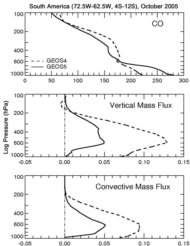
Fig. 12. Vertical profiles of CO (top), total air mass flux (middle), and convective mass flux (bottom) in October 2005 at the center of the biomass burning region in South America ( 72.5^{\circ}\text{W} – 62.5^{\circ}\text{W} , 4^{\circ}\text{S} – 12^{\circ}\text{S} ) for simulations driven by GEOS-4 (dashed) and GEOS-5 (solid). Mass flux is in \text{Pa s}^{-1} , CO is in ppb.
