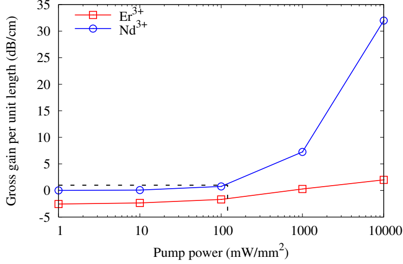
Fig. 7. Local gross gain per unit length at the center of the active layer and in the beginning of the waveguide as a function of the pumping power for a waveguide doped with \text{Nd}^{3+} (open circle) and a waveguide doped with \text{Er}^{3+} (open square) recorded at x = 4.5 \mu\text{m} and y = 8.55 \mu\text{m} (center of the XY section of the active layer) and z = 0 (beginning of the waveguide). Losses found by Pirasteh et al [8] are represented (dashed line).
