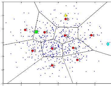
FIGURE 1.1 Soft quantization and sparse coding.
