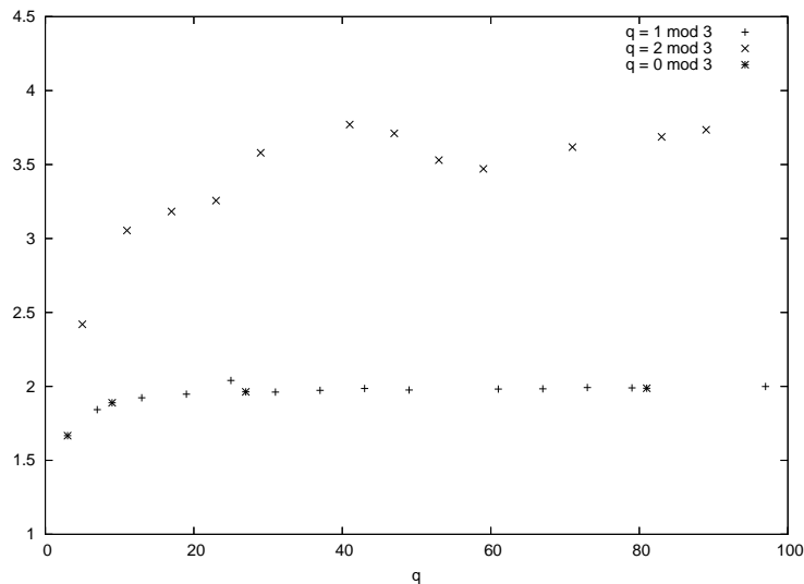
FIGURE 1. The value of \frac{1}{q} \max_{b \in L^\times} R_L(bx^d) where L has order q^2 and q \leq 100 .
