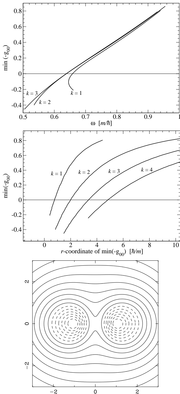
FIG. 10. The first and second panel shows the value of the minimum of -g_{00} for free-field boson stars of different rotational quantum number k , as a function of \omega and the location of the minimum, respectively. Isocontours of -g_{00} in a plane of constant (t, \varphi) are plotted in the third panel, for k = 2 and \omega = 0.55 m/\hbar . The Cartesian-like coordinates of this plot are x := r \sin \theta and z := r \cos \theta , in units of \hbar/m . The ergoregion is the torus shown in dashed-lines.
