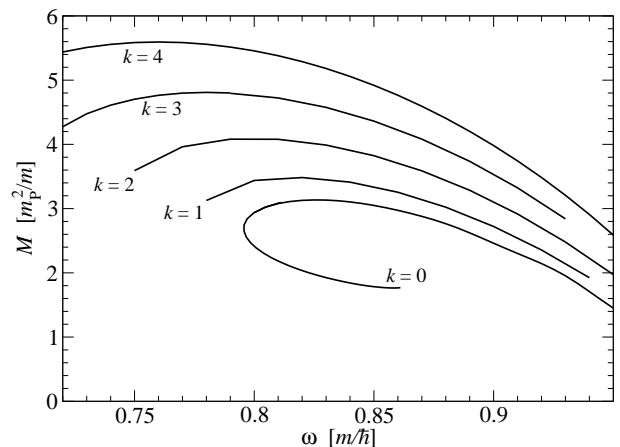
FIG. 11. Gravitational mass as a function of \omega for boson star models constructed upon the self-interacting potential (5) with \Lambda = 200 , with different values of the rotational quantum number k .
