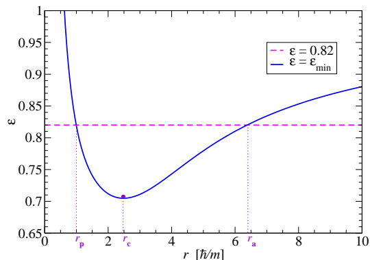
FIG. 14. Effective potential profile for \ell = 1 \hbar/m . Only the region where \varepsilon \geq \varepsilon_{\min} is allowed for the motion of the test particle, so the radial coordinate r must obey r_p \leq r \leq r_a . The spot marks the position of the stable circular orbit of radius r_c .
