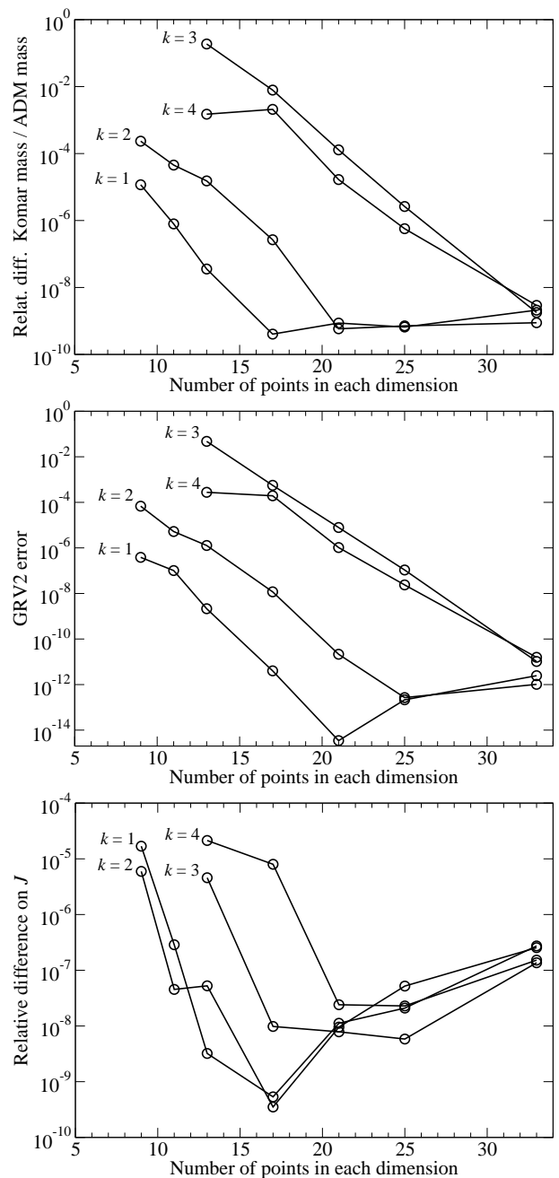
FIG. 5. Various error indicators as the number of spectral coefficients in both the radial and angular dimensions, for configurations with \omega = 0.8 m/\hbar and rotational quantum number k = 1, 2, 3 and 4. The first panel shows the error on the masses, the second one on the GRV2 identity and the last one on the angular momentum.
