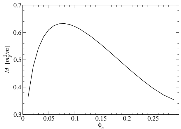
FIG. 3. Gravitational mass M as a function of \phi_c for spherical configurations and a free scalar field.
