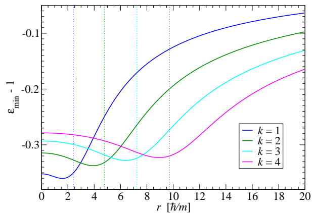
FIG. 20. Effective potential for \ell = 0 and for rotating boson stars with \omega = 0.8 m/\hbar and different values of k . The vertical lines mark the position of the maximum of the scalar field modulus for each boson star.
