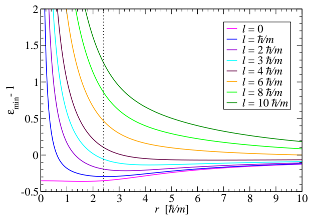
FIG. 13. Effective potential profiles for a free-field rotating boson star with \omega = 0.8m/\hbar and k = 1 . The vertical line represents the location of maximum of the scalar field modulus \phi (cf. Fig. 8).
