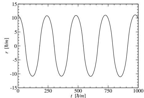
FIG. 21. Evolution of the r -coordinate of a \ell = 0 test particle of initially at rest at r_i = 10.79 \hbar/m in the spacetime generated by a spherical ( k = 0 ) boson star with \omega = 0.77 m/\hbar .
