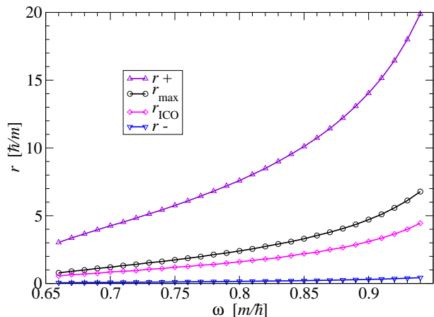
FIG. 16. Innermost circular orbit radius r_{\text{ICO}} as a function of \omega for boson stars with k = 1 . r_{\text{max}} is the location of the maximum of the scalar field modulus \phi , while r_+ and r_- denote to the radii where \phi = \phi_{\text{max}}/10 .
