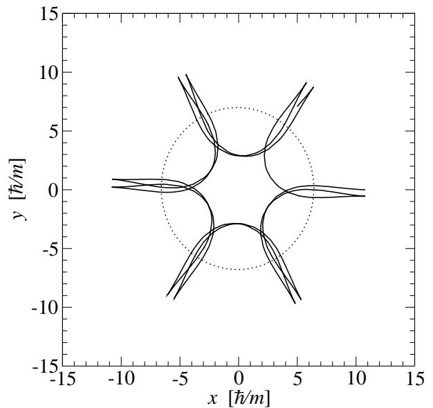
FIG. 24. Same as Fig. 22 but for k = 3 .
