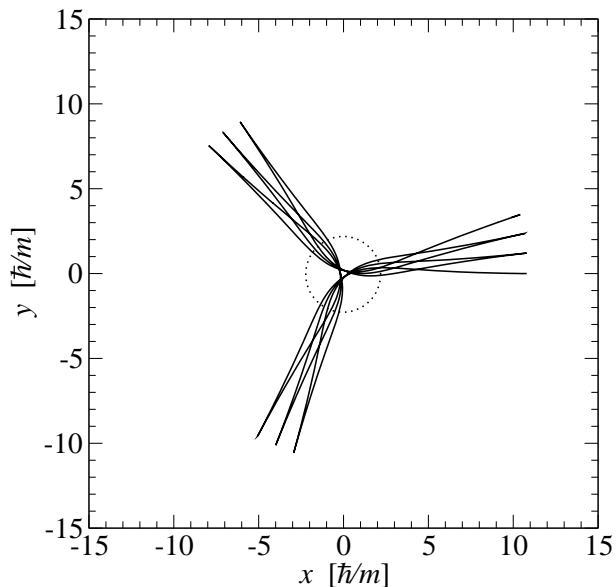
FIG. 22. Orbit of a \ell = 0 test particle in the equatorial plane of a rotating free-field boson star with k = 1 and \omega = 0.80m/\hbar ; the particle is initially at rest at r = r_i = 10.79\hbar/m and \varphi = 0 . The Cartesian-like coordinates of the plot are x := r \cos \varphi and y := r \sin \varphi . The dotted circle marks the maximum of the scalar field modulus \phi .
