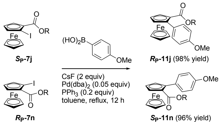
Scheme 8. Suzuki cross-couplings from 2-iodoferrocenecarboxylates S P -7j and R P -7n .
