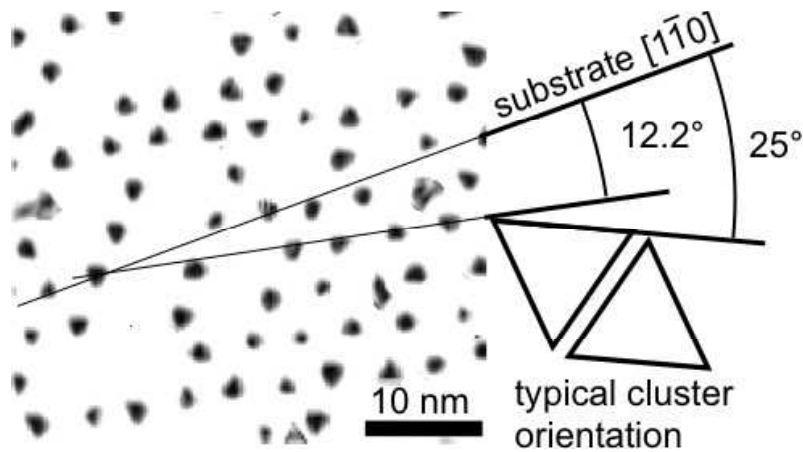
Fig. 11. Processed STM image of 0.23 nm Pd clusters deposited at RT. The substrate [1 \bar{1} 0] has been identified on a large scale STM image from the same experiment where both oxide orientations were present. The typical orientation of the Pd clusters is 25^\circ related to the close-packed \text{Ni}_3\text{Al} rows.
