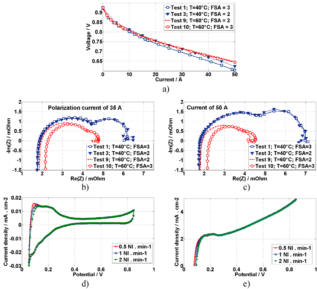
Fig. 4 - Effects of anode flow rate on the FC performances.
