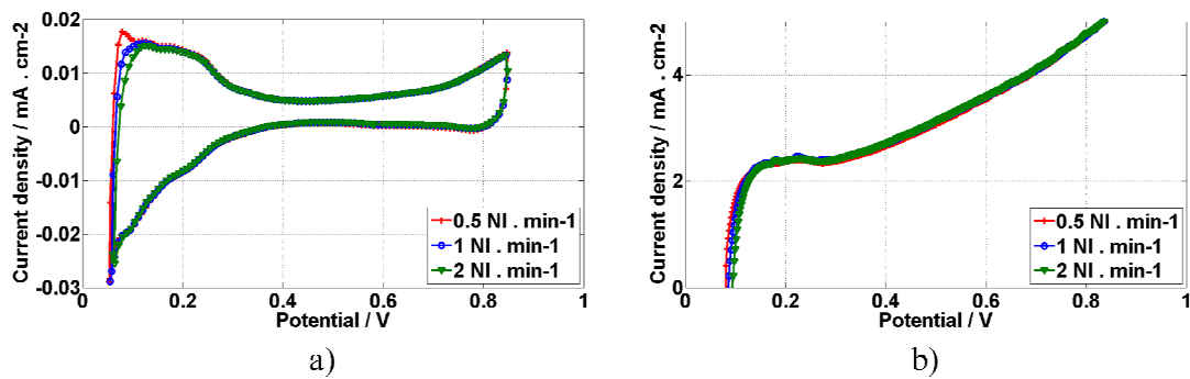
Fig. 2 - Example of hydrogen and nitrogen flow rate effects on the CV (Fig. 2a) and LSV (Fig. 2b) diagrams (case: Tests 1, 2, 3).
