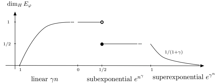
FIGURE 1. \dim_H E_\varphi for different \varphi .
