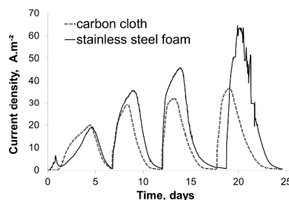
Fig. 1: Variation of current density with time for carbon cloth and stainless steel foam bioanodes polarized at -0.2 \text{ V/SCE} .
