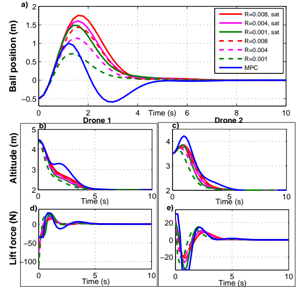
Fig. 4. Saturated and non-saturated LQR with different weighting matrices
