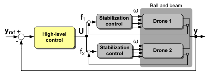
Fig. 2. Control scheme
