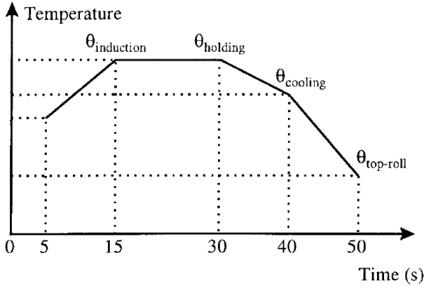
Fig. 5. Thermal cycle.
