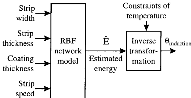
Fig. 6. Estimation of the induction temperature.
