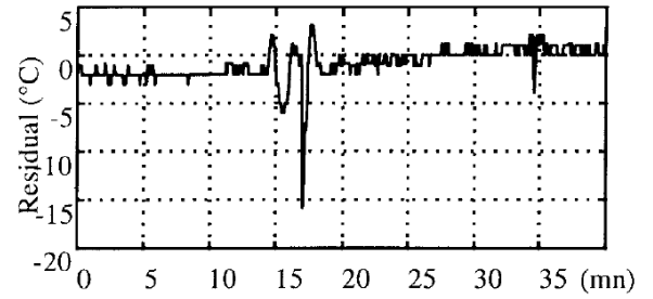
Fig. 4. Example of residual for \theta_{induction} .
