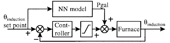
Fig. 12. Control architecture for \theta_{induction} .
