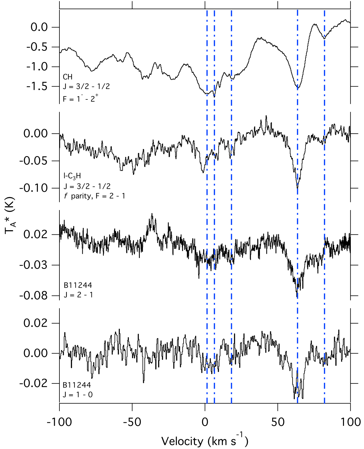
Fig. 3.— Observed transitions of B11244 and l\text{-C}_3\text{H} toward Sgr B2(N) from PRIMOS and CH toward Sgr B2(N) from HEXOS. The blue vertical lines are provided to guide the eye to the diffuse cloud velocity components. The velocity axis is referenced to the rest frequency of each transition.
