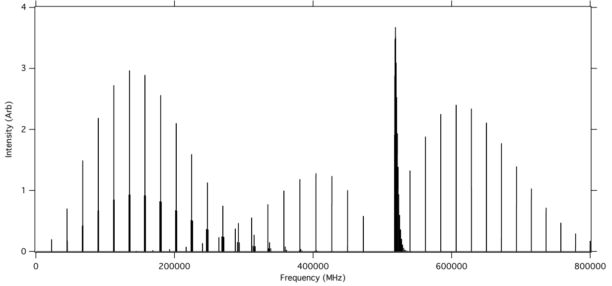
Fig. 1.— Simulated spectrum of \text{C}_3\text{H}^- at LTE, with an excitation temperature of T_{ex} = 22 K.
