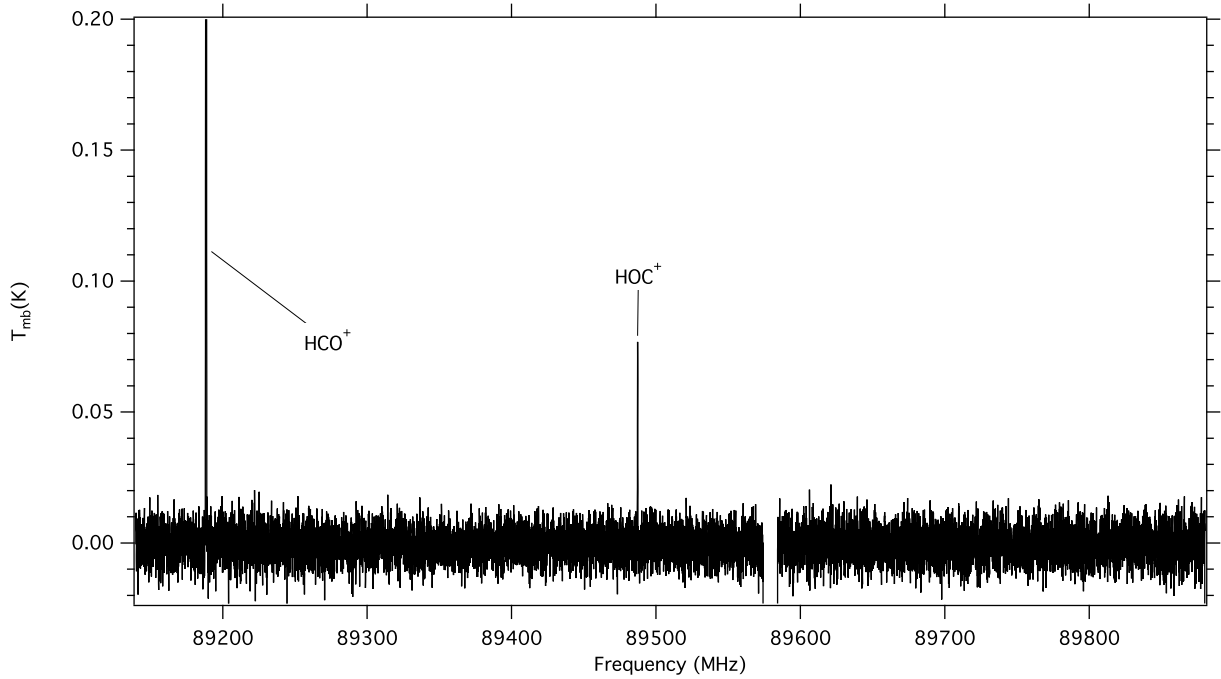
Fig. 2.— Targeted frequency window around the predicted K_a = 1, 4_{1,4} - 3_{1,3} transition of C_3H^- centered at 89535 MHz. The RMS noise level is 5.8 mK. Three features are observed - one each attributed to HCO^+ and HOC^+ . A third, located at \sim 89580 MHz, has been positively identified as belonging to a known interstellar species, but has been removed from the spectra for proprietary reasons. The identity of this line will be published in a forthcoming paper from Guzmán et al.
