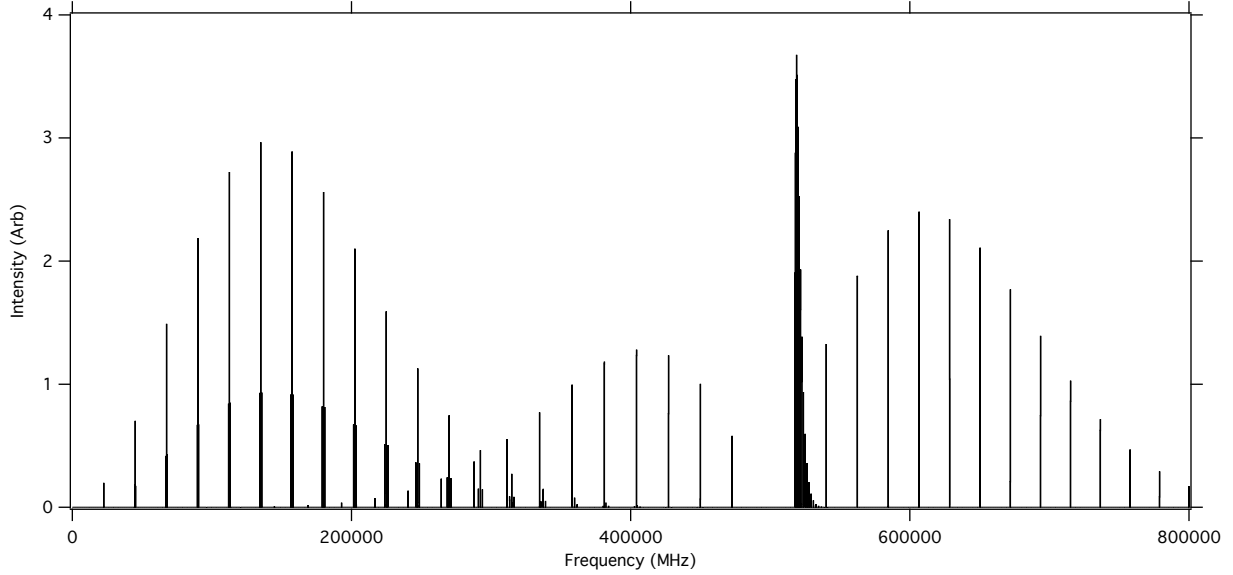
Fig. 1.— Simulated spectrum of C_3H^- at LTE, with an excitation temperature of T_{ex} = 22 K.
