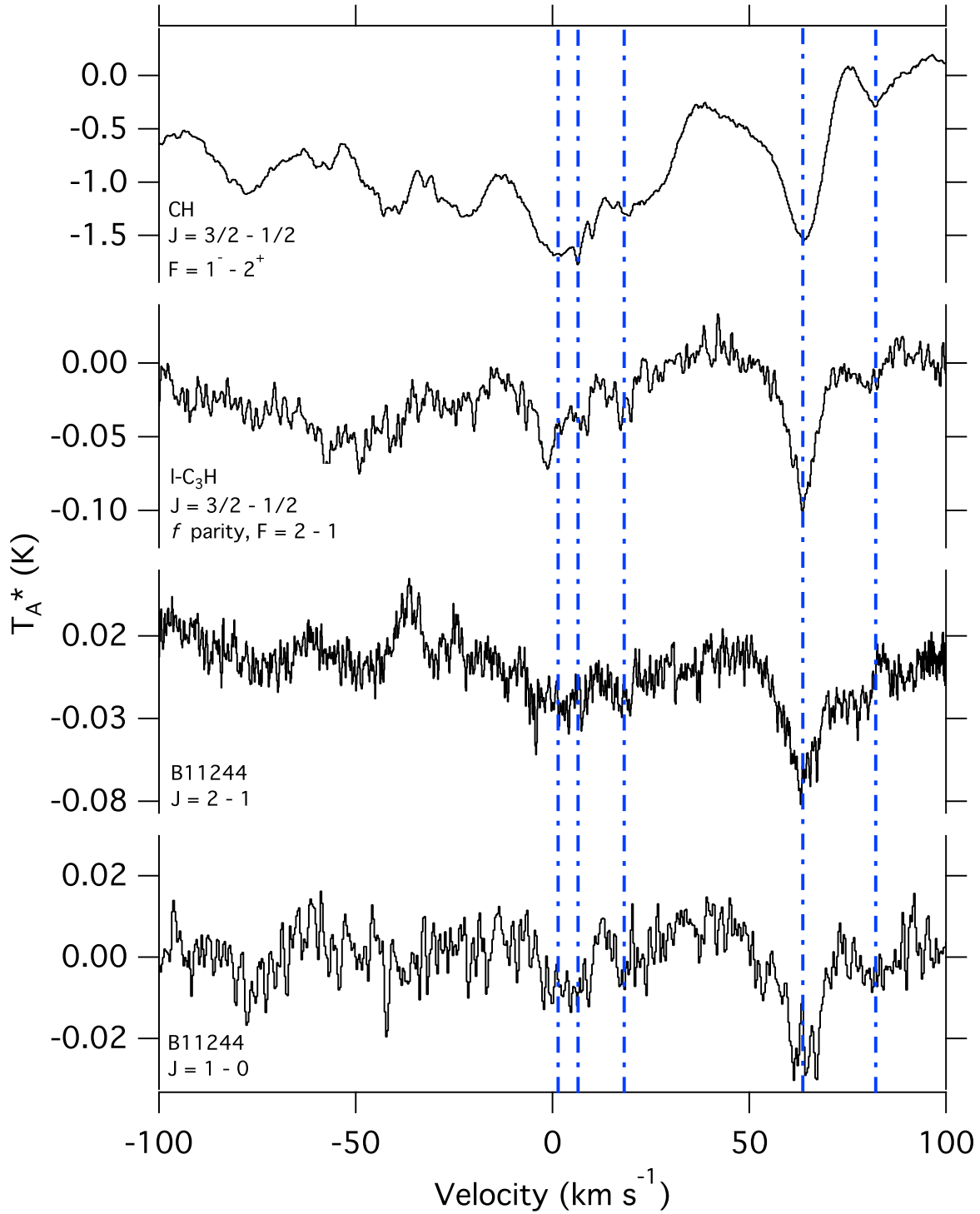
Fig. 3.— Observed transitions of B11244 and l -C 3 H toward Sgr B2(N) from PRIMOS and CH toward Sgr B2(N) from HEXOS. The blue vertical lines are provided to guide the eye to the diffuse cloud velocity components. The velocity axis is referenced to the rest frequency of each transition.
