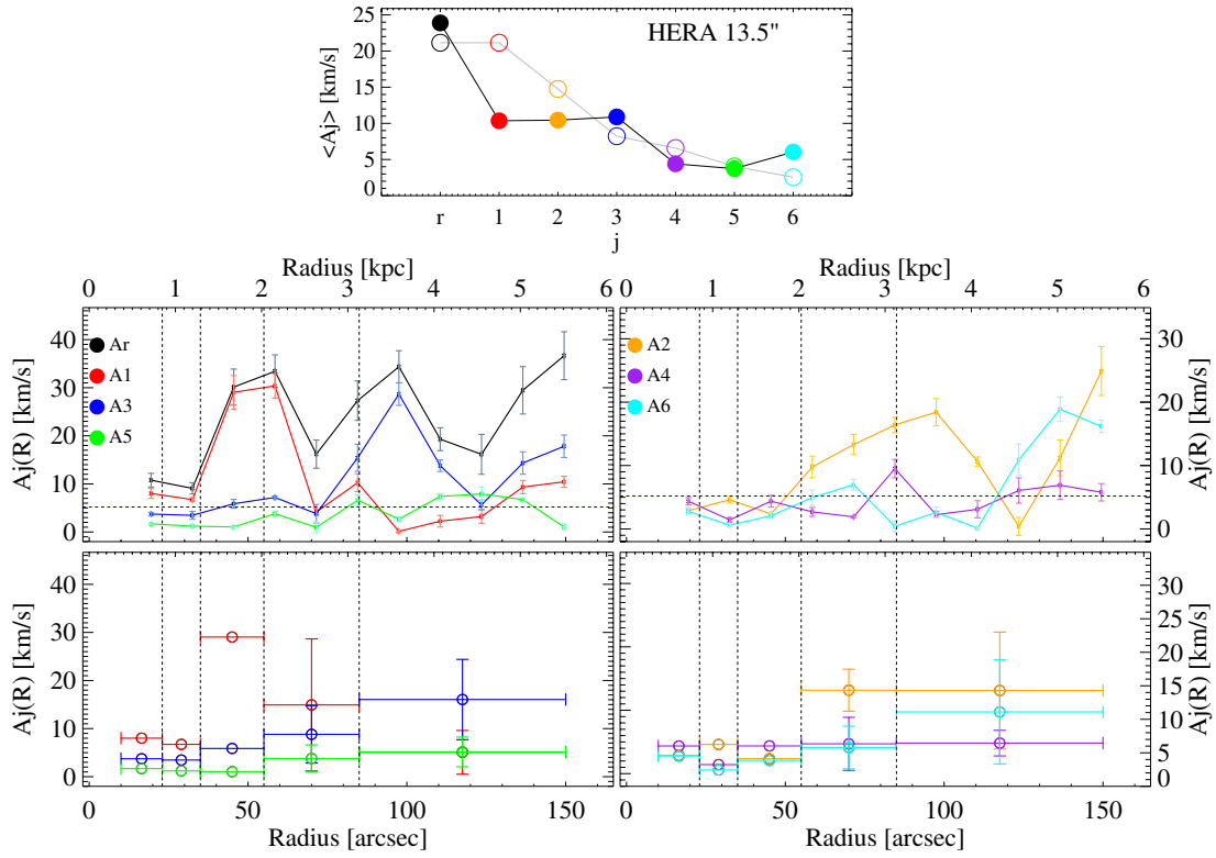
Figure 10. Top: radially averaged mean of the harmonic component amplitudes A_j from HERACLES 13''5 residual velocity field. Open dots indicate the measurements restricted on the PAWS FoV. Bottom: non-circular motion amplitudes from harmonic decomposition; radial trend of the odd components and the total power A_r(R) (top left) and even components (top right). The horizontal blue dashed straight line indicates twice the channel width of the data cube, i.e., 2 \times 2.6 \text{ km s}^{-1} = 5.2 \text{ km s}^{-1} . In the bottom row the mean behavior of the odd (left) and even (middle) components in the different M51 environments as defined in Meidt et al. (2013) (dashed vertical lines; see the text for details) are indicated together with the standard deviations of the values. Horizontal error bars represents the widths of the environments.
