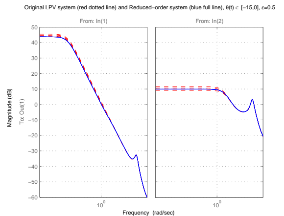
Fig. 1. Frozen Bode plots of (1) original controller: LPV system with LFT on one parameter (dashed line) and (2) reduced controller: LTI system (full line).
