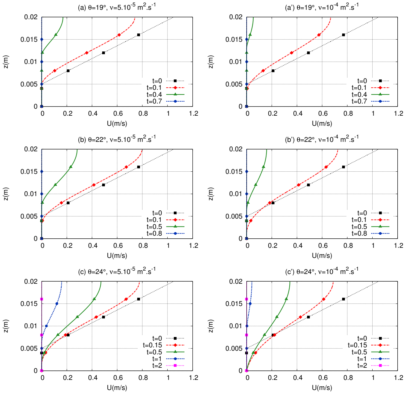
Figure 11: Velocity profiles U(Z) at different times, with a linear velocity profile, for two different viscosities (a-b-c) \nu = 5 \times 10^{-5} \text{m}^2 \text{s}^{-1} and (a'-b'-c') \nu = 10^{-4} \text{m}^2 \text{s}^{-1} , and for the slope angles (a-a') \theta = 19^\circ , (b-b') \theta = 22^\circ , and (c-c') \theta = 24^\circ .
