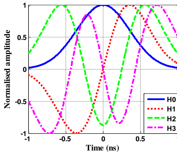
Figure 8: Hermite functions, orders n = 0 to 3.
