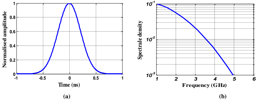
Figure 3: Gaussian pulse – time (a) and spectrum (b) representations.
