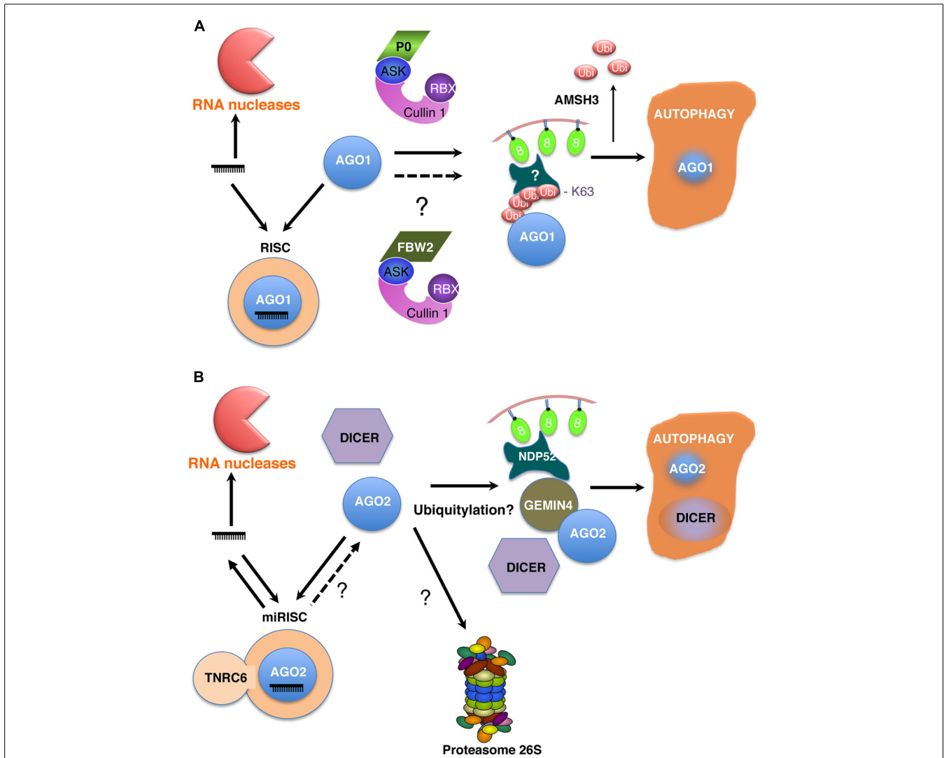
FIGURE 1 | Models for the turnover of AGO proteins in Arabidopsis (A) and mammalian cells (B). Different levels of regulation operate on the homeostasis of RISCs. First, the steady-state levels of microRNAs are regulated by degradation processes involving different ribonucleases (RNases) acting either 3′–5′ or 5′–3′. Thus microRNAs most likely are in competition for AGO binding. Recent evidences essentially from metazoans indicate that at least some microRNAs can be released from RISCs, explaining their short half-lives. However, not only microRNAs but also AGO proteins are degraded. Thus in both plants and animal cells, it is now clearly established that AGO proteins are degraded by autophagy in an RNA free form prior RISC assembly. This mechanism also co-degrades other
