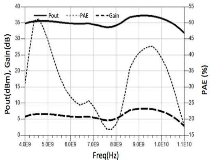
Fig. 7. Input matched Simulated Pout, PAE and Gain @Pin=29dBm
