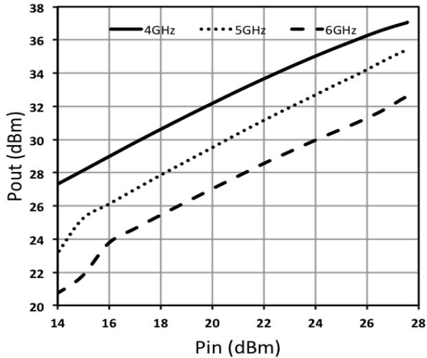
Fig. 4. Measured Pout vs. Pin @4GHz, 5GHz and 6GHz
