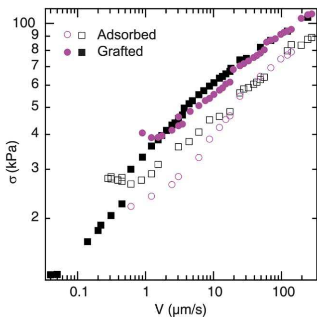
Fig. 6 Comparison between the friction stress on end grafted chains and irreversibly adsorbed chains. The filled symbols correspond to grafted chains. The open symbols correspond to irreversibly adsorbed chains. ● 43 kg mol -1 grafted, ○ 50 kg mol -1 adsorbed ■ 107 kg mol -1 grafted □ 105 kg mol -1 adsorbed.
