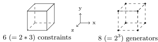
Fig. 3. Constraint and generator representations of the 3-dimensional hypercube
