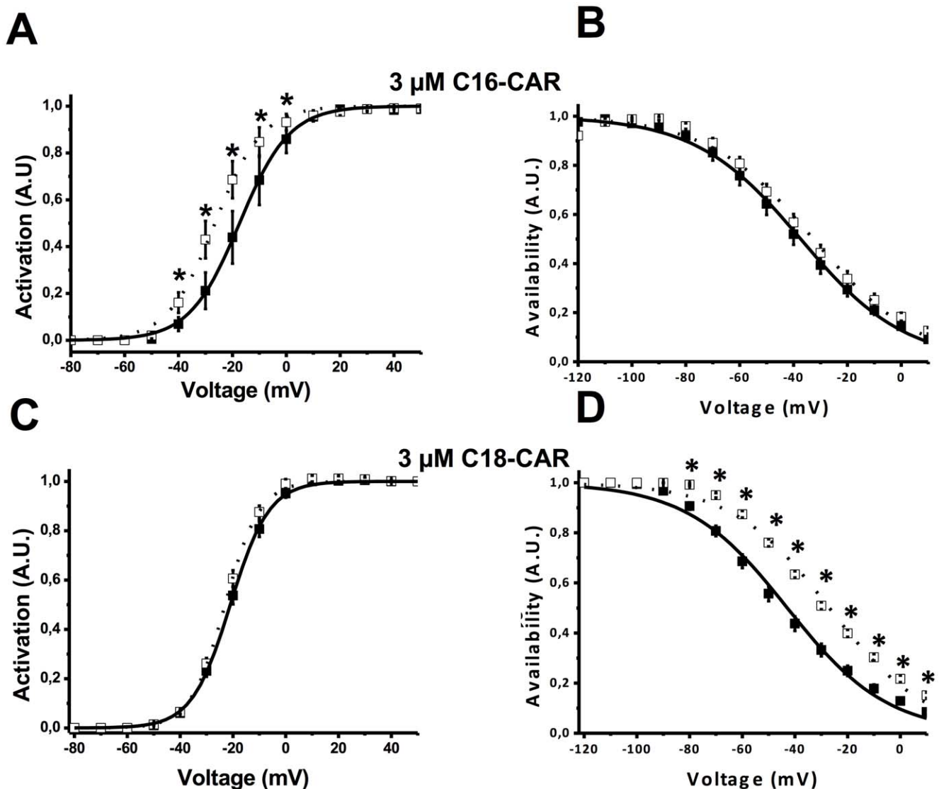
Figure 2. Effect of extracellular long-chain acyl-CARs on the activation and availability of the hERG current. A , effect of 3 \mu M C16-CAR on the activation curve. In the absence of C16-CAR (filled squares, n=6 cells), the V_{1/2} is -17.4 \pm 0.2 mV while in the presence of 3 \mu M acyl-CAR (empty squares) the V_{1/2} is -26.5 \pm 0.5 mV. B , effect of 3 \mu M C16-CAR on availability. In the absence of C16-CAR (empty squares, n=6 cells), the V_{1/2} is -35.4 \pm 1.4 mV while in the presence of 3 \mu M acyl-CAR (filled squares) the V_{1/2} is -37.4 \pm 0.5 mV. C , effect of 3 \mu M C18-CAR on activation. In the absence of C18-CAR (filled squares, n=7 cells), the V_{1/2} is -21.0 \pm 0.1 mV while in the presence of 3 \mu M acyl-CAR (empty squares) the V_{1/2} is -23.0 \pm 0.2 mV. D , effect of 3 \mu M C18-CAR on availability. In the absence of C18-CAR (filled squares, n=7 cells) the V_{1/2} is -42.9 \pm 1.0 mV while in the presence of 3 \mu M acyl-CAR (empty squares) the V_{1/2} is -27.0 \pm 1.0 mV. * : p < 0.01 . doi:10.1371/journal.pone.0041686.g002
