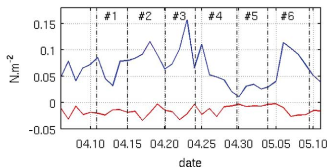
Figure 2. Time evolution of the wind stress alongshore (blue line) and cross-shore (red line) components (in \text{N m}^{-2} ) near 14^\circ\text{S} , 77^\circ\text{W} from ASCAT scatterometer during the glider deployment. The dates corresponding to each glider cross-shore section are marked by dashed vertical lines.
