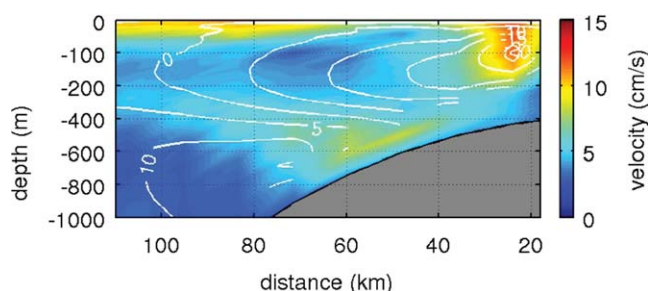
Figure 5. Vertical section (at 14^{\circ}\text{S} ) of the standard deviation associated with the model composite at t = 0 days. White lines represent the alongshore velocities from the composite at t = 0 days.
