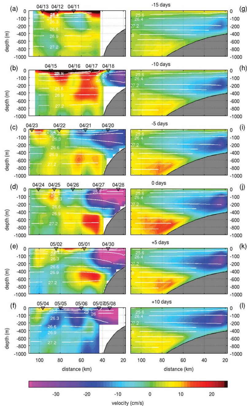
Figure 3. (a–f) Alongshore geostrophic velocity near 14°S (perpendicular to each glider sections) objectively mapped. White lines represent the isopycnals of the original data. (g–l) Alongshore velocity composite from the regional model simulation at 14°S. The criteria used to build the composite are detailed in section 2. White lines represent the isopycnals. The depth axis is not linear in order to highlight the top 200 m of the sections. The horizontal axis represents the distance from the coast.
