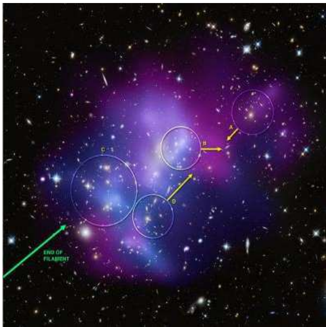
Fig. 6. MACS J0717.5 + 3745 : Chandra colour image on HST showing galaxies in 4 different clusters involved in collision, with direction of motion for three fastest moving clusters. The length of the arrow shows the approximate speed in a direction perpendicular to the line of sight. The direction of motion of the cluster appears roughly parallel to the direction of the filament (Credit: X-ray (NASA/CXC/I f A/C.Maetal.2008,2009); Optical (NASA/STScI/I f A/C.Maetal.2008,2009)).
