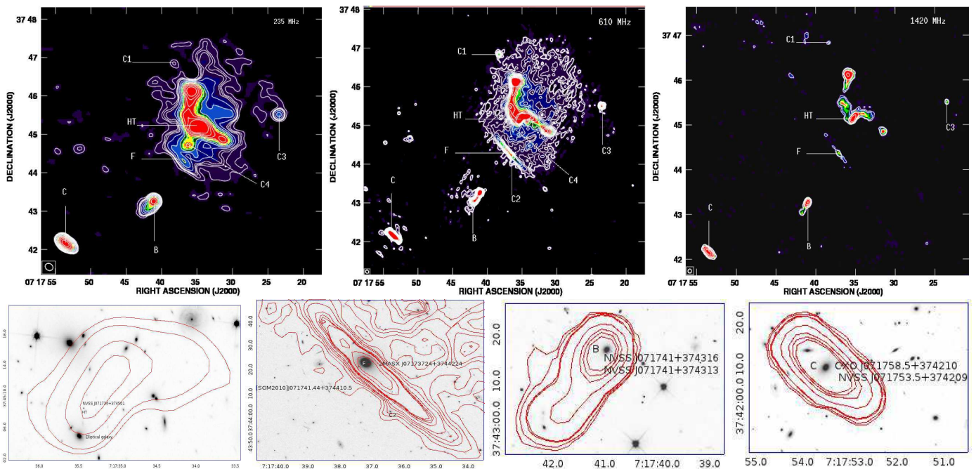
Fig. 1. High resolution radio images of massive galaxy cluster MACS J0717.5 + 3745 ( z = 0.5548 ) at 0.235 GHz ( Top left ) at FWHM beam of 13.46'' \times 10.76'' resolution, 0.61 GHz ( Top middle ) at FWHM of 5.70'' \times 4.82'' resolution and 1.42 GHz ( Top right ) at FWHM of 5'' \times 5'' resolution. Contours start at (3\sigma) and scale by a factor of \sqrt{2} . Bottom panels : Finding charts from HST for source HT, F ( z = 0.1546 ), B and C with overlaid 0.61 GHz radio contours.
