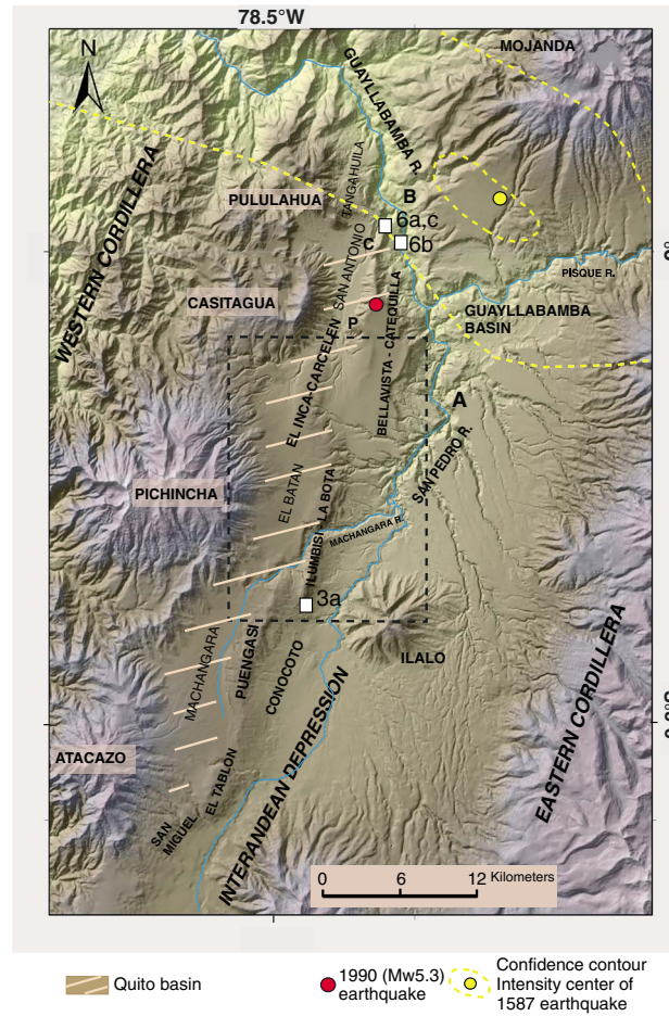
Figure 2. DEM 20 m topographic map and Quaternary settings of Quito region: the toponymy used in the text is reported together with volcanic edifices, tectonic segments, and principal rivers. Black frame corresponds to Figure 4 extent. Maximum intensity area for the historical earthquake Guayllabamba 1587 (6.4 M_c \sim M_w ). The confidence contours are related to the probability (51 and 95%) that the maximum intensity is inside this area [Beauval et al., 2010]. White squares correspond to Figures 6a–6c and 3a. The red dot corresponds to 08 November 1990 ( M_w 5.3) earthquake. C: Catequilla andesitic dome and P: Pacpo dacitic dome.
