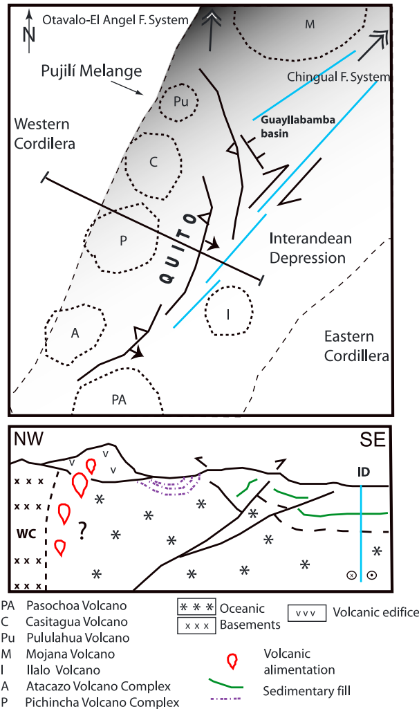
Figure 10. Simplified kinematic model for active deformation in Quito region. Interpretations after the geometry of mapped fault systems in plane view, seismicity, and GPS data as presented in previous figures. ID: Interandean Depression; WC: Western Cordillera
