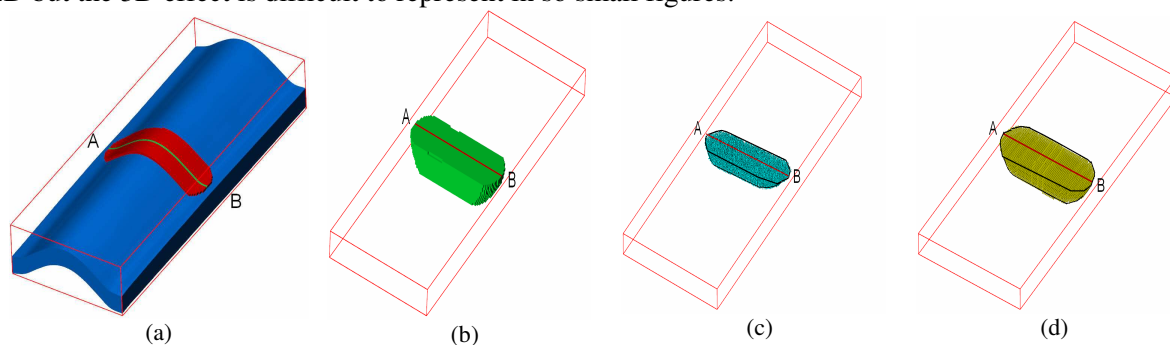
Figure 4: Distance measured in resulting grid between two points A and B: (a) lithostratigraphic grid; (b) flattened by the traditional method; (c) by the vertical shear, (d) by the isometric.
